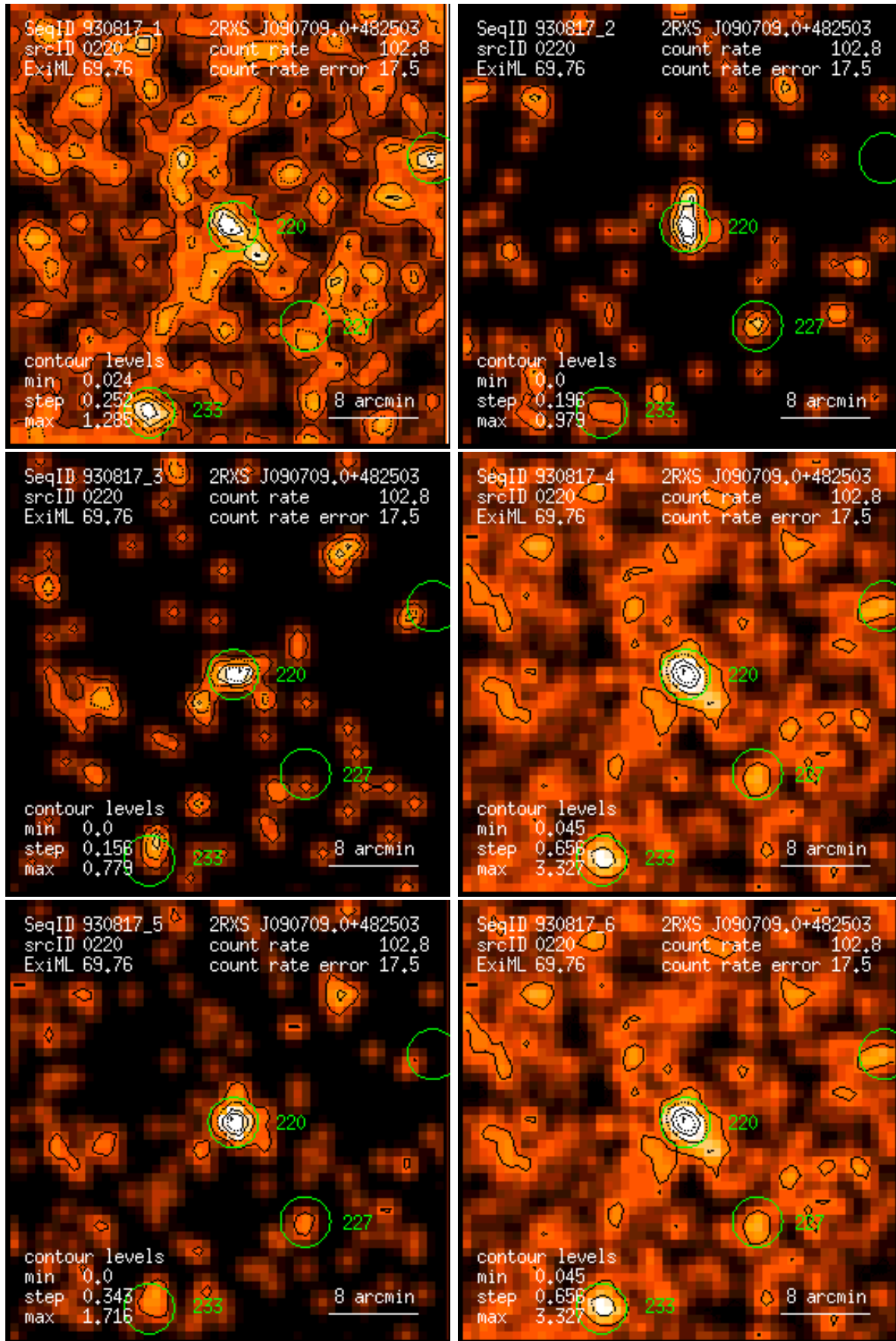
Figure 220: RASS 930817: detection 0220: band rate images, Gaussian filter: (1) PSPC channels 11 – 41, (2) 52 – 90, (3) 91 – 201, (4) 11 – 235, (5) 52 – 201, (6) 11 – 201. Broad band rates in counts/ks. Band rate contour levels in counts/ks/arcmin 2 .
