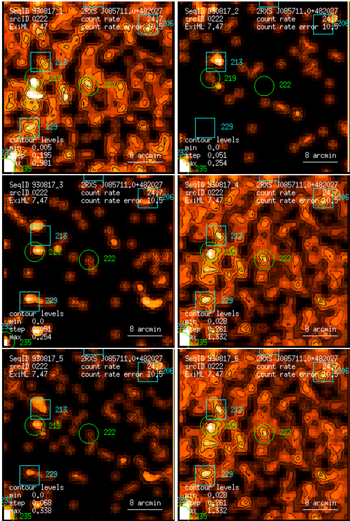
Figure 222: RASS 930817: detection 0222: band rate images, Gaussian filter: (1) PSPC channels 11 – 41, (2) 52 – 90, (3) 91 – 201, (4) 11 – 235, (5) 52 – 201, (6) 11 – 201. Broad band rates in counts/ks. Band rate contour levels in counts/ks/arcmin 2 .
