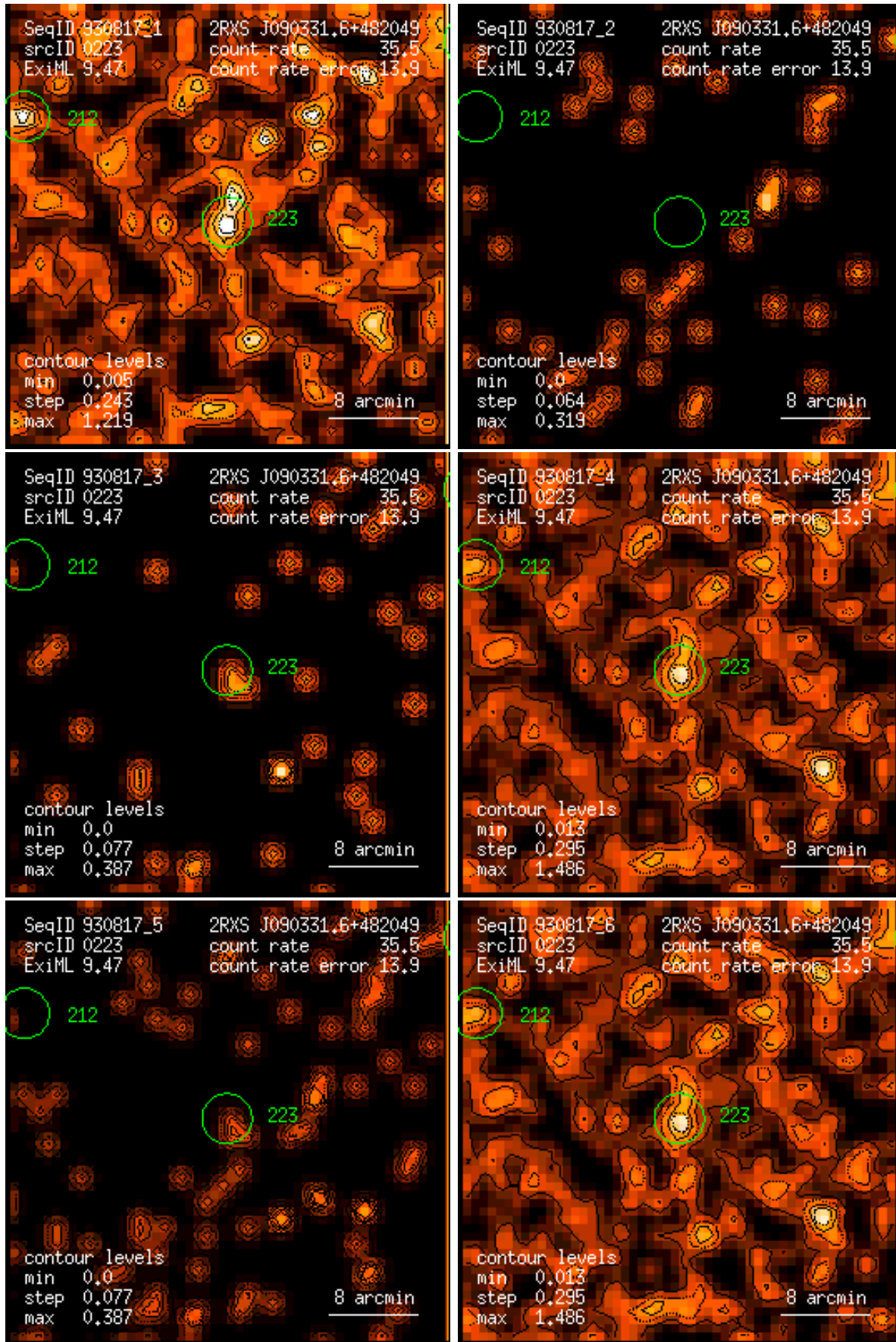
Figure 223: RASS 930817: detection 0223: band rate images, Gaussian filter: (1) PSPC channels 11 – 41, (2) 52 – 90, (3) 91 – 201, (4) 11 – 235, (5) 52 – 201, (6) 11 – 201. Broad band rates in counts/ks. Band rate contour levels in counts/ks/arcmin 2 .
