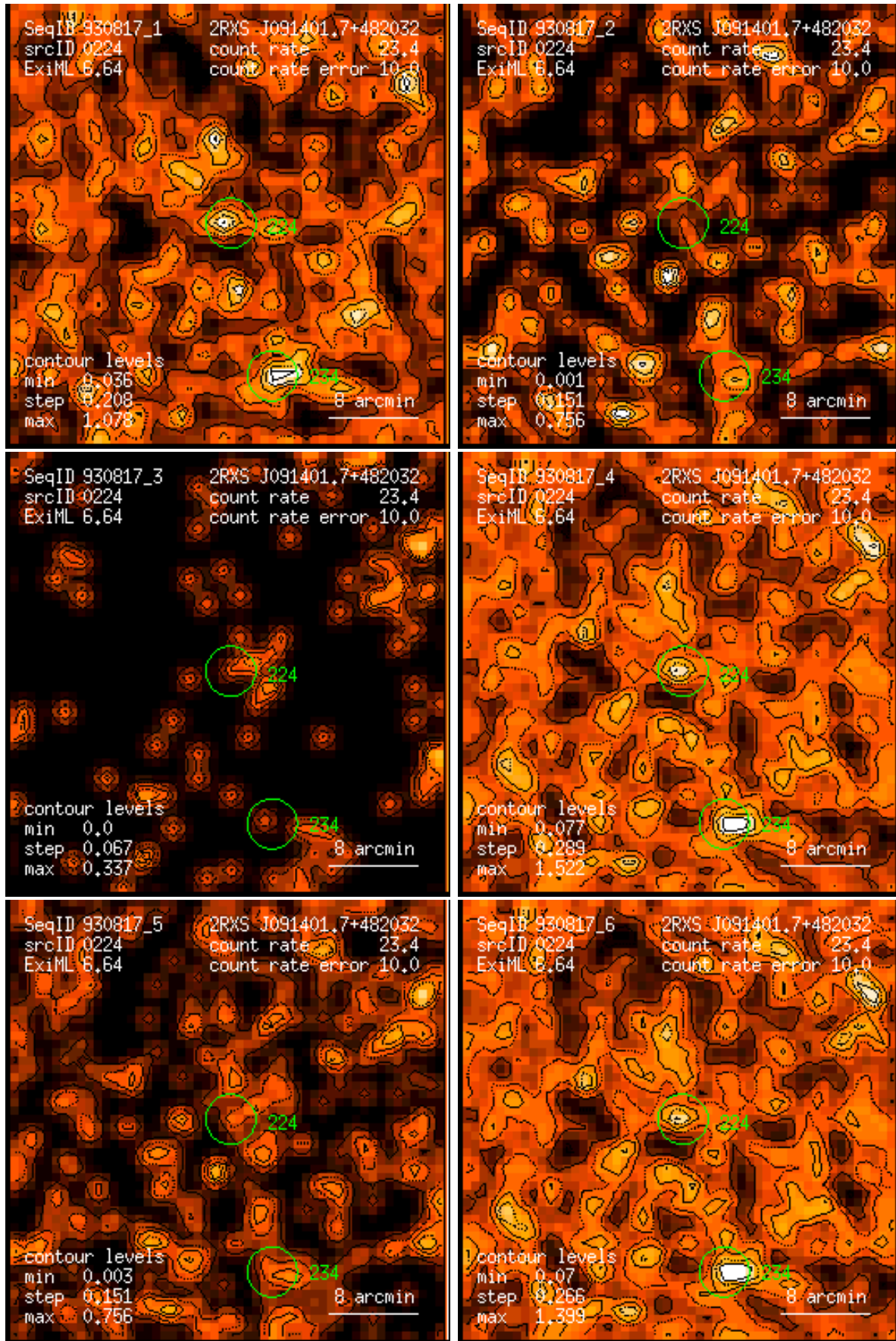
Figure 224: RASS 930817: detection 0224: band rate images, Gaussian filter: (1) PSPC channels 11 – 41, (2) 52 – 90, (3) 91 – 201, (4) 11 – 235, (5) 52 – 201, (6) 11 – 201. Broad band rates in counts/ks. Band rate contour levels in counts/ks/arcmin 2 .
