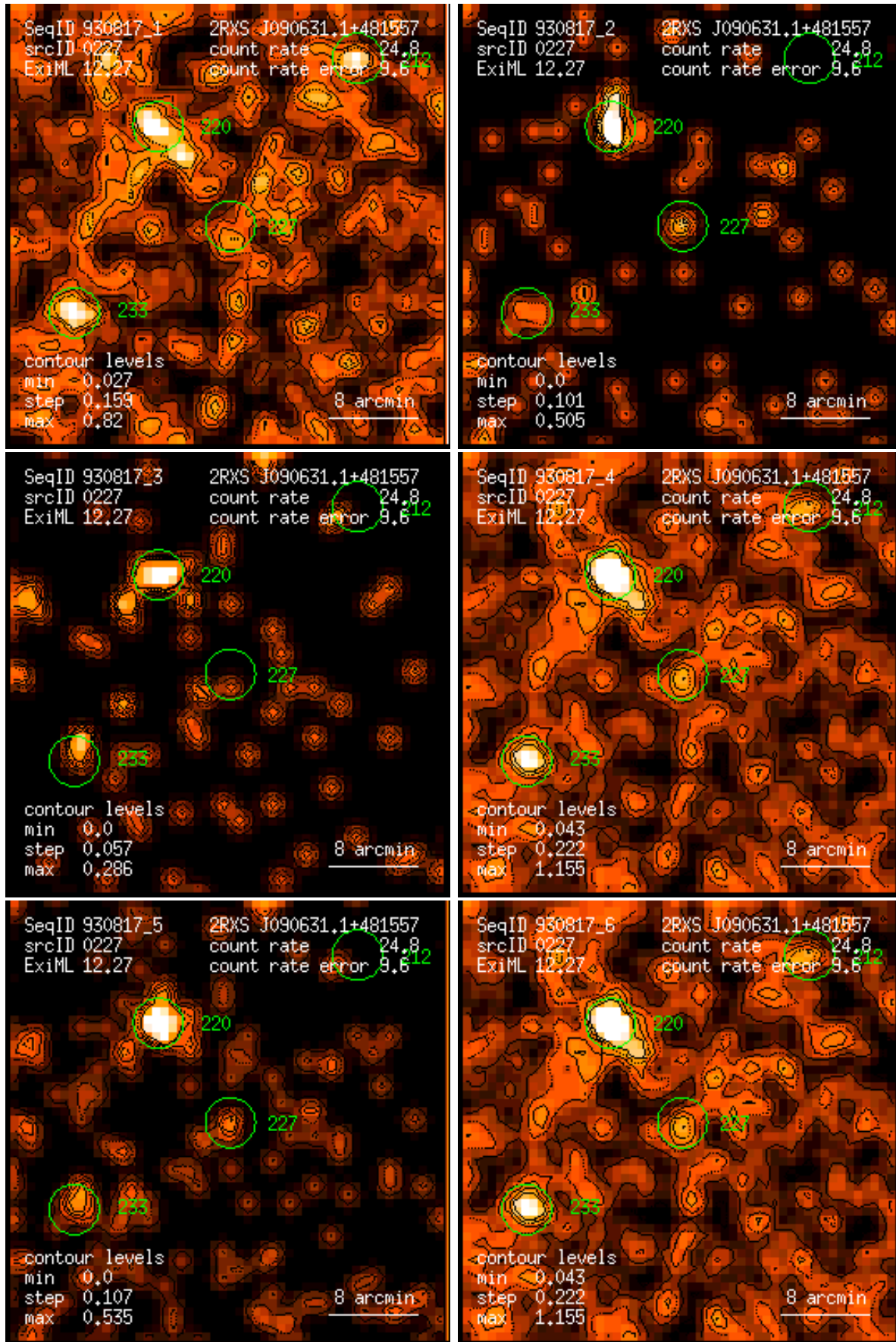
Figure 227: RASS 930817: detection 0227: band rate images, Gaussian filter: (1) PSPC channels 11 – 41, (2) 52 – 90, (3) 91 – 201, (4) 11 – 235, (5) 52 – 201, (6) 11 – 201. Broad band rates in counts/ks. Band rate contour levels in counts/ks/arcmin 2 .
