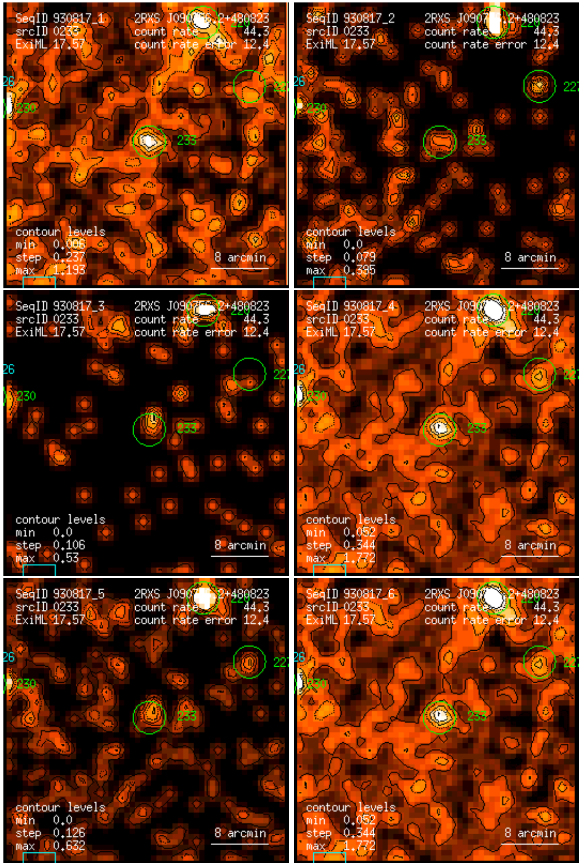
Figure 233: RASS 930817: detection 0233: band rate images, Gaussian filter: (1) PSPC channels 11 – 41, (2) 52 – 90, (3) 91 – 201, (4) 11 – 235, (5) 52 – 201, (6) 11 – 201. Broad band rates in counts/ks. Band rate contour levels in counts/ks/arcmin 2 .
