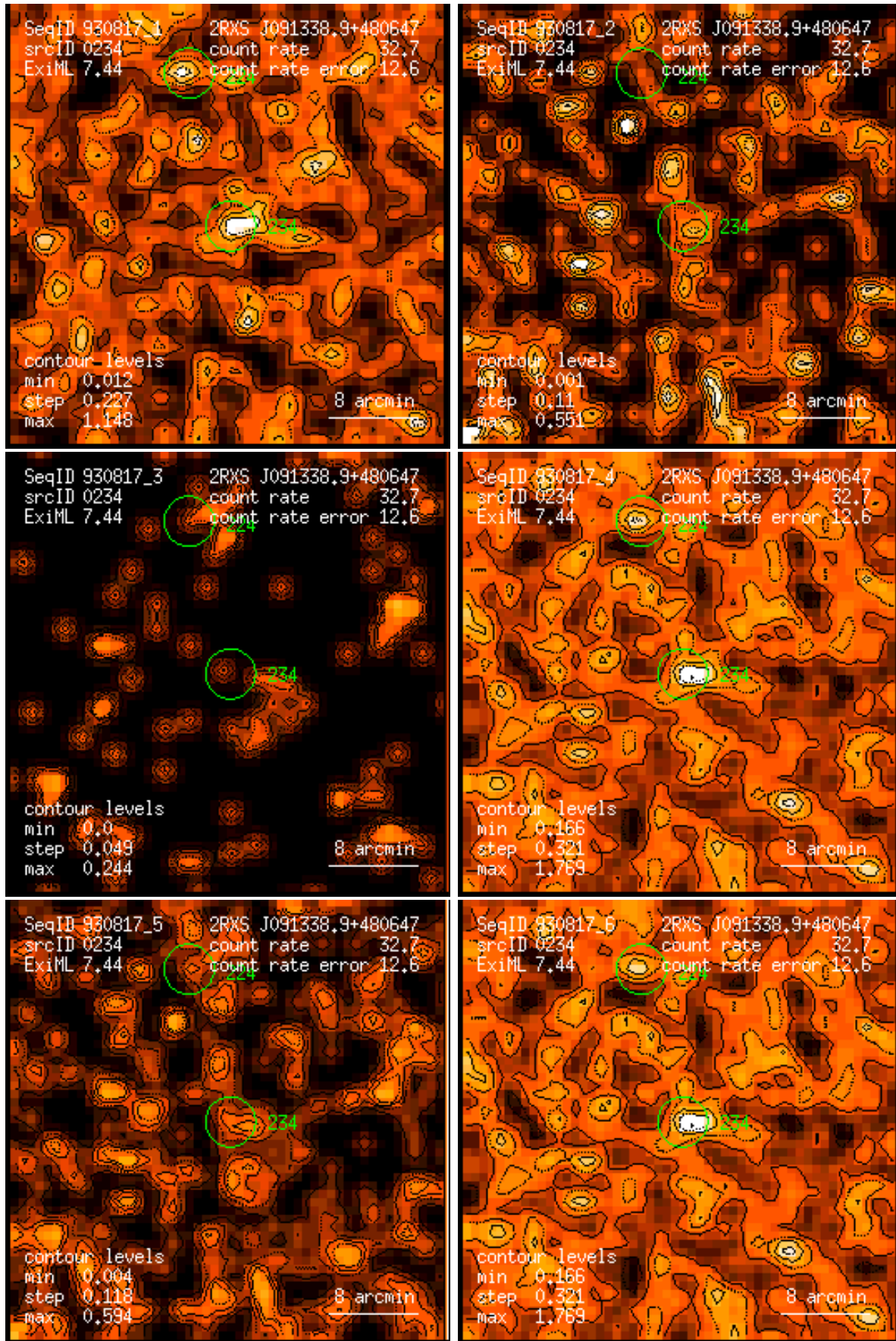
Figure 234: RASS 930817: detection 0234: band rate images, Gaussian filter: (1) PSPC channels 11 – 41, (2) 52 – 90, (3) 91 – 201, (4) 11 – 235, (5) 52 – 201, (6) 11 – 201. Broad band rates in counts/ks. Band rate contour levels in counts/ks/arcmin 2 .
