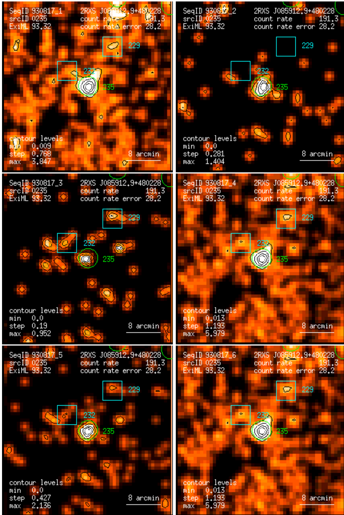
Figure 235: RASS 930817: detection 0235: band rate images, Gaussian filter: (1) PSPC channels 11 – 41, (2) 52 – 90, (3) 91 – 201, (4) 11 – 235, (5) 52 – 201, (6) 11 – 201. Broad band rates in counts/ks. Band rate contour levels in counts/ks/arcmin 2 .
