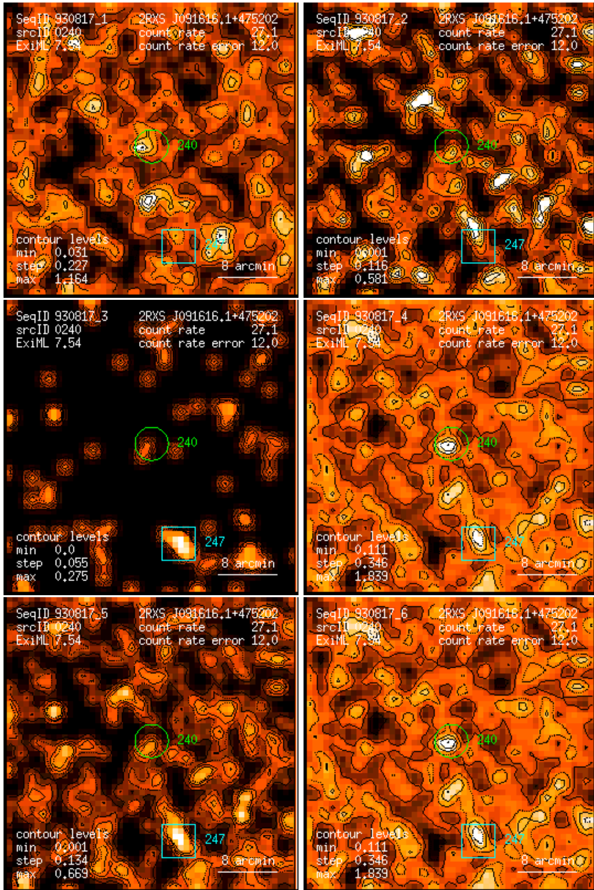
Figure 240: RASS 930817: detection 0240: band rate images, Gaussian filter: (1) PSPC channels 11 – 41, (2) 52 – 90, (3) 91 – 201, (4) 11 – 235, (5) 52 – 201, (6) 11 – 201. Broad band rates in counts/ks. Band rate contour levels in counts/ks/arcmin 2 .
