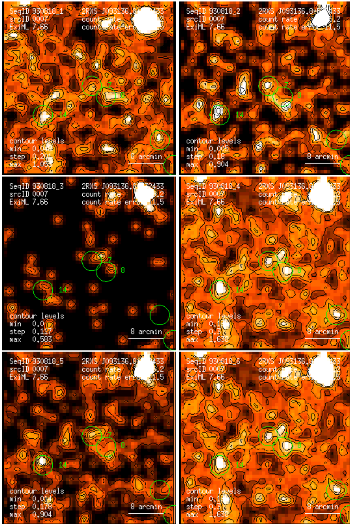
Figure 7: RASS 930818: detection 0007: band rate images, Gaussian filter: (1) PSPC channels 11 – 41, (2) 52 – 90, (3) 91 – 201, (4) 11 – 235, (5) 52 – 201, (6) 11 – 201. Broad band rates in counts/ks. Band rate contour levels in counts/ks/arcmin 2 .
