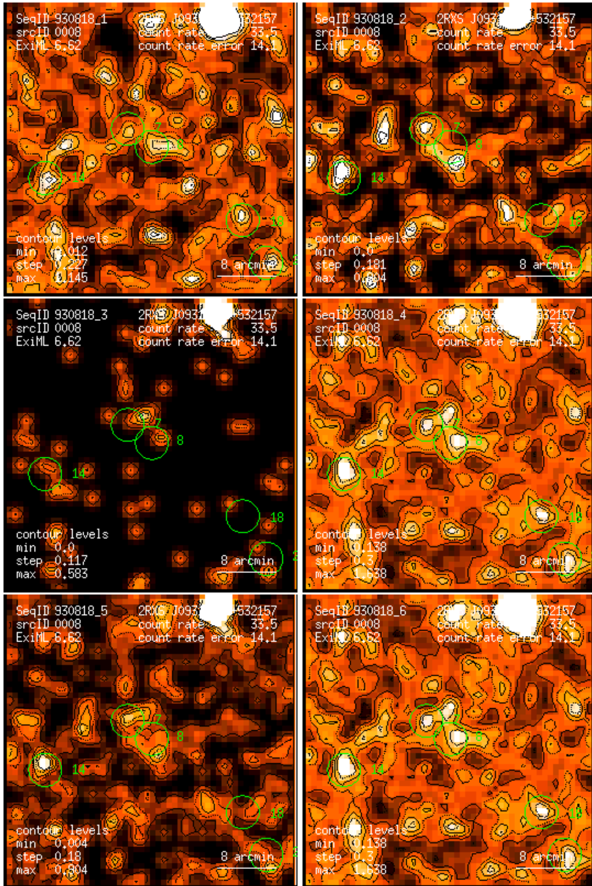
Figure 8: RASS 930818: detection 0008: band rate images, Gaussian filter: (1) PSPC channels 11 – 41, (2) 52 – 90, (3) 91 – 201, (4) 11 – 235, (5) 52 – 201, (6) 11 – 201. Broad band rates in counts/ks. Band rate contour levels in counts/ks/arcmin 2 .
