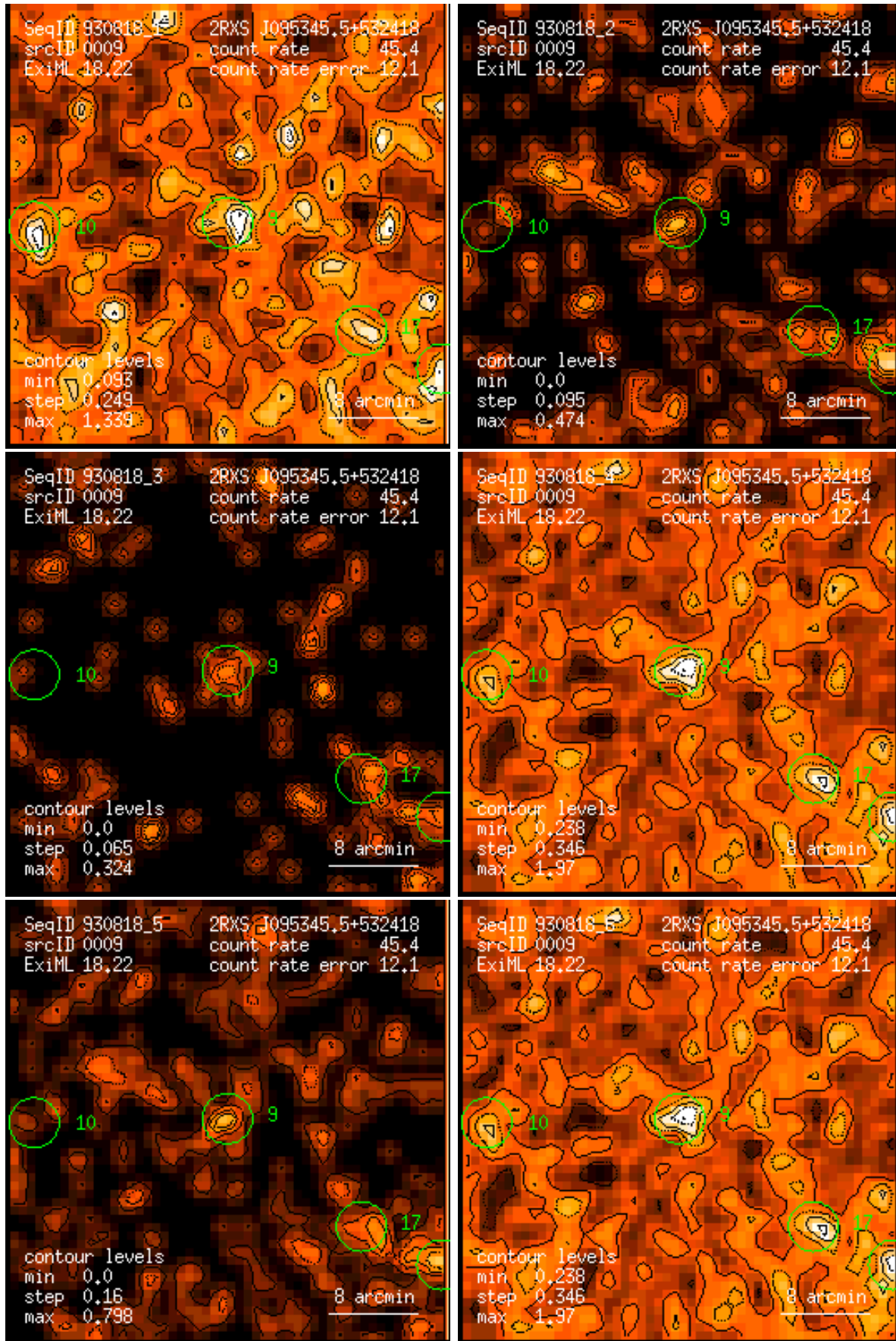
Figure 9: RASS 930818: detection 0009: band rate images, Gaussian filter: (1) PSPC channels 11 – 41, (2) 52 – 90, (3) 91 – 201, (4) 11 – 235, (5) 52 – 201, (6) 11 – 201. Broad band rates in counts/ks. Band rate contour levels in counts/ks/arcmin 2 .
