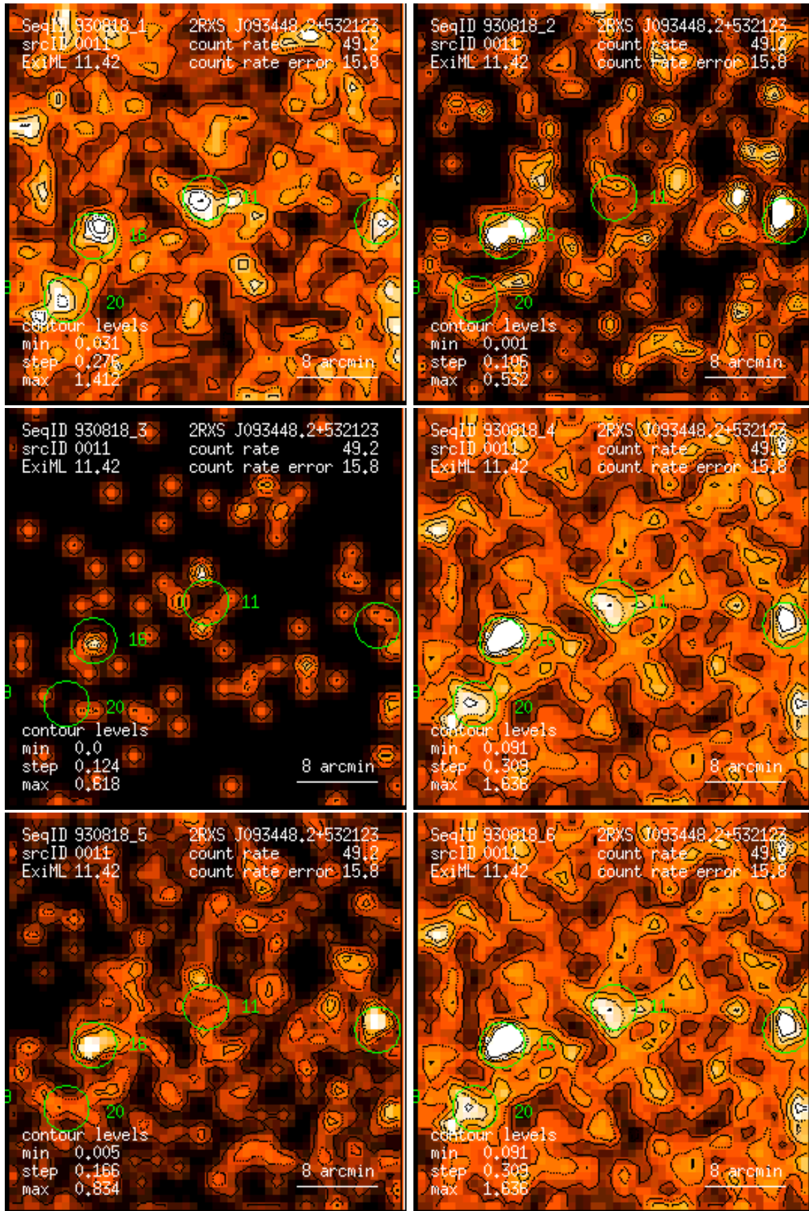
Figure 11: RASS 930818: detection 0011: band rate images, Gaussian filter: (1) PSPC channels 11 – 41, (2) 52 – 90, (3) 91 – 201, (4) 11 – 235, (5) 52 – 201, (6) 11 – 201. Broad band rates in counts/ks. Band rate contour levels in counts/ks/arcmin 2 .
