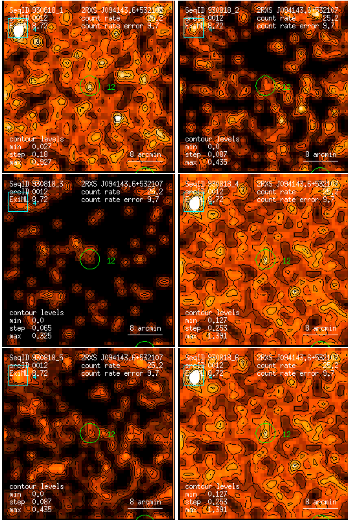
Figure 12: RASS 930818: detection 0012: band rate images, Gaussian filter: (1) PSPC channels 11 – 41, (2) 52 – 90, (3) 91 – 201, (4) 11 – 235, (5) 52 – 201, (6) 11 – 201. Broad band rates in counts/ks. Band rate contour levels in counts/ks/arcmin 2 .
