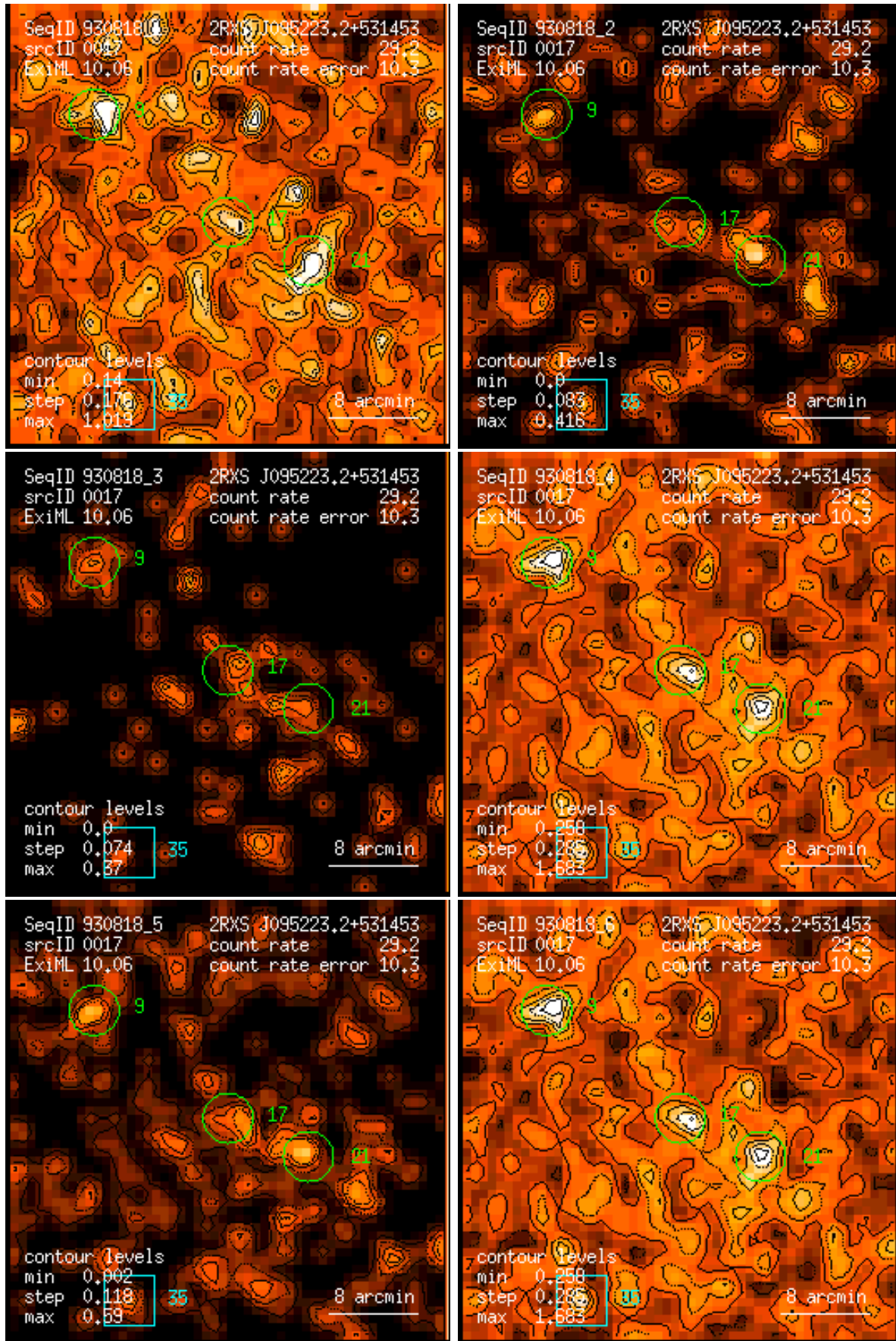
Figure 17: RASS 930818: detection 0017: band rate images, Gaussian filter: (1) PSPC channels 11 – 41, (2) 52 – 90, (3) 91 – 201, (4) 11 – 235, (5) 52 – 201, (6) 11 – 201. Broad band rates in counts/ks. Band rate contour levels in counts/ks/arcmin 2 .
