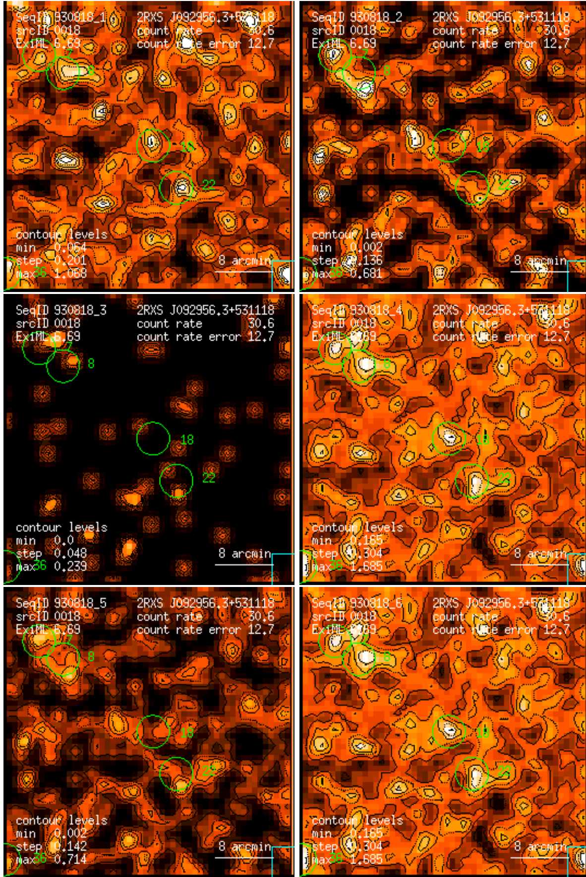
Figure 18: RASS 930818: detection 0018: band rate images, Gaussian filter: (1) PSPC channels 11 – 41, (2) 52 – 90, (3) 91 – 201, (4) 11 – 235, (5) 52 – 201, (6) 11 – 201. Broad band rates in counts/ks. Band rate contour levels in counts/ks/arcmin 2 .
