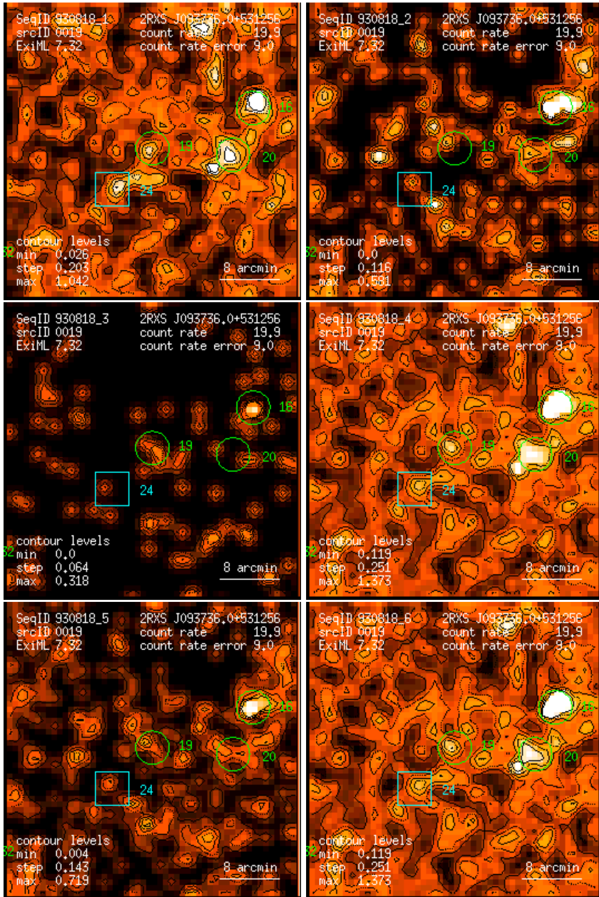
Figure 19: RASS 930818: detection 0019: band rate images, Gaussian filter: (1) PSPC channels 11 – 41, (2) 52 – 90, (3) 91 – 201, (4) 11 – 235, (5) 52 – 201, (6) 11 – 201. Broad band rates in counts/ks. Band rate contour levels in counts/ks/arcmin 2 .
