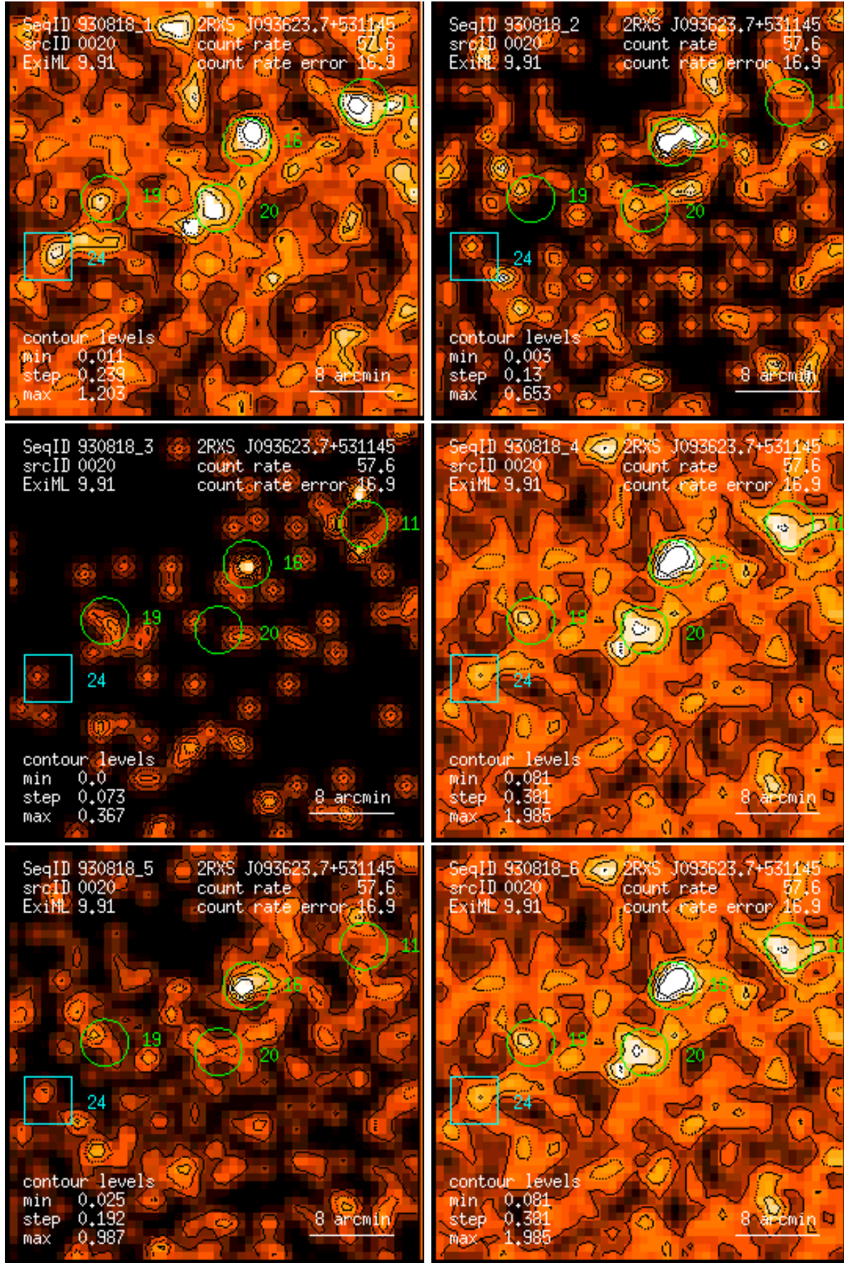
Figure 20: RASS 930818: detection 0020: band rate images, Gaussian filter: (1) PSPC channels 11 – 41, (2) 52 – 90, (3) 91 – 201, (4) 11 – 235, (5) 52 – 201, (6) 11 – 201. Broad band rates in counts/ks. Band rate contour levels in counts/ks/arcmin 2 .
