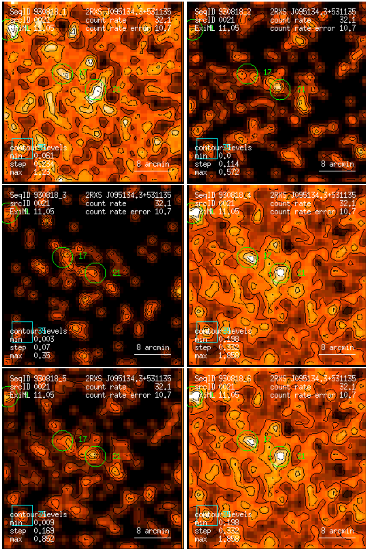
Figure 21: RASS 930818: detection 0021: band rate images, Gaussian filter: (1) PSPC channels 11 – 41, (2) 52 – 90, (3) 91 – 201, (4) 11 – 235, (5) 52 – 201, (6) 11 – 201. Broad band rates in counts/ks. Band rate contour levels in counts/ks/arcmin 2 .
