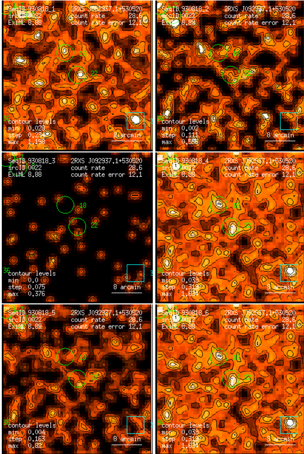
Figure 22: RASS 930818: detection 0022: band rate images, Gaussian filter: (1) PSPC channels 11 – 41, (2) 52 – 90, (3) 91 – 201, (4) 11 – 235, (5) 52 – 201, (6) 11 – 201. Broad band rates in counts/ks. Band rate contour levels in counts/ks/arcmin 2 .
