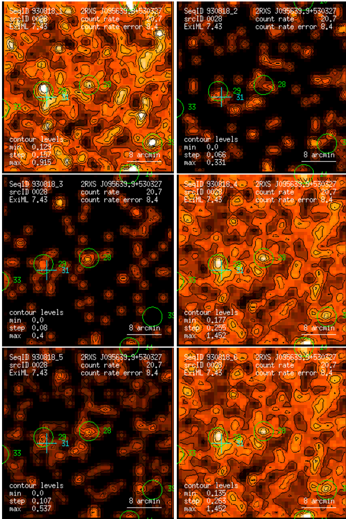
Figure 28: RASS 930818: detection 0028: band rate images, Gaussian filter: (1) PSPC channels 11 – 41, (2) 52 – 90, (3) 91 – 201, (4) 11 – 235, (5) 52 – 201, (6) 11 – 201. Broad band rates in counts/ks. Band rate contour levels in counts/ks/arcmin 2 .
