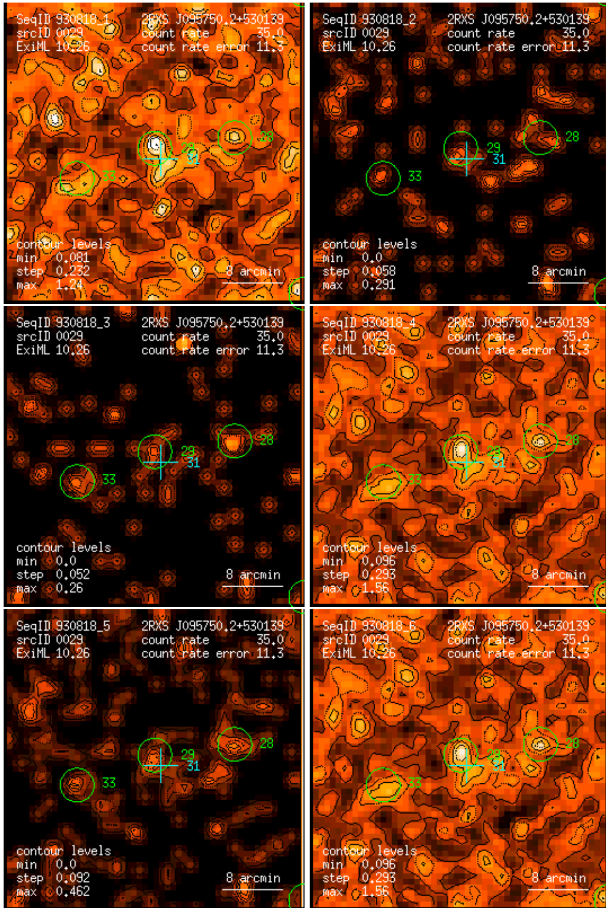
Figure 29: RASS 930818: detection 0029: band rate images, Gaussian filter: (1) PSPC channels 11 – 41, (2) 52 – 90, (3) 91 – 201, (4) 11 – 235, (5) 52 – 201, (6) 11 – 201. Broad band rates in counts/ks. Band rate contour levels in counts/ks/arcmin 2 .
