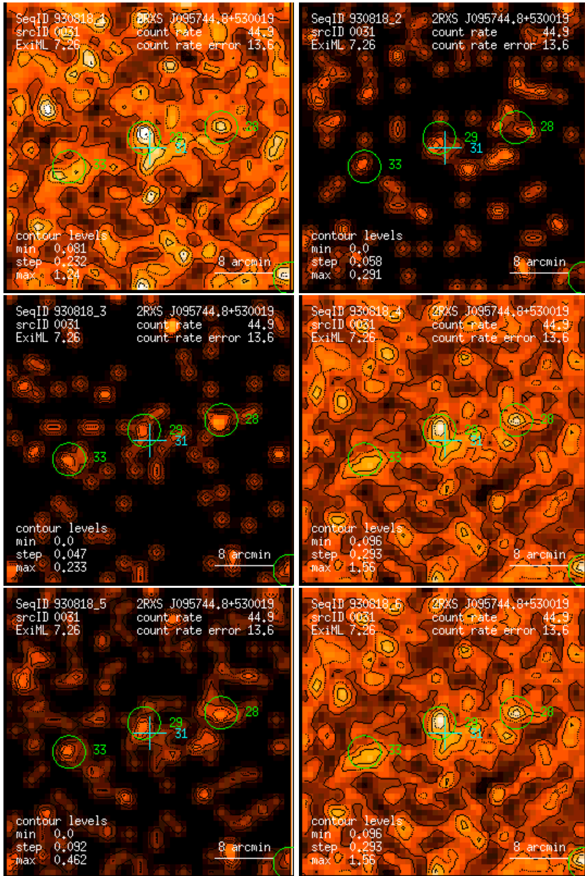
Figure 31: RASS 930818: detection 0031: band rate images, Gaussian filter: (1) PSPC channels 11 – 41, (2) 52 – 90, (3) 91 – 201, (4) 11 – 235, (5) 52 – 201, (6) 11 – 201. Broad band rates in counts/ks. Band rate contour levels in counts/ks/arcmin 2 .
