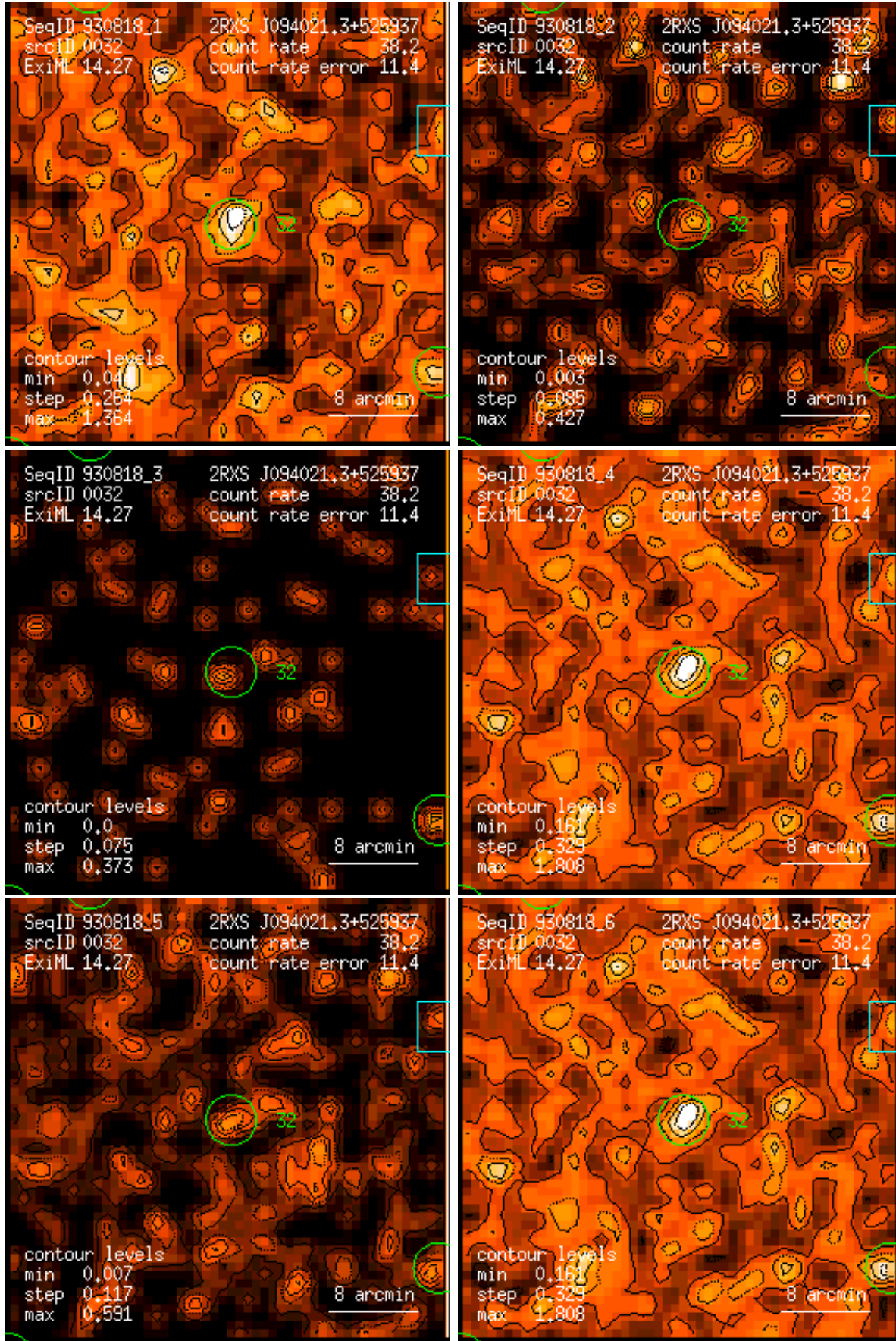
Figure 32: RASS 930818: detection 0032: band rate images, Gaussian filter: (1) PSPC channels 11 – 41, (2) 52 – 90, (3) 91 – 201, (4) 11 – 235, (5) 52 – 201, (6) 11 – 201. Broad band rates in counts/ks. Band rate contour levels in counts/ks/arcmin 2 .
