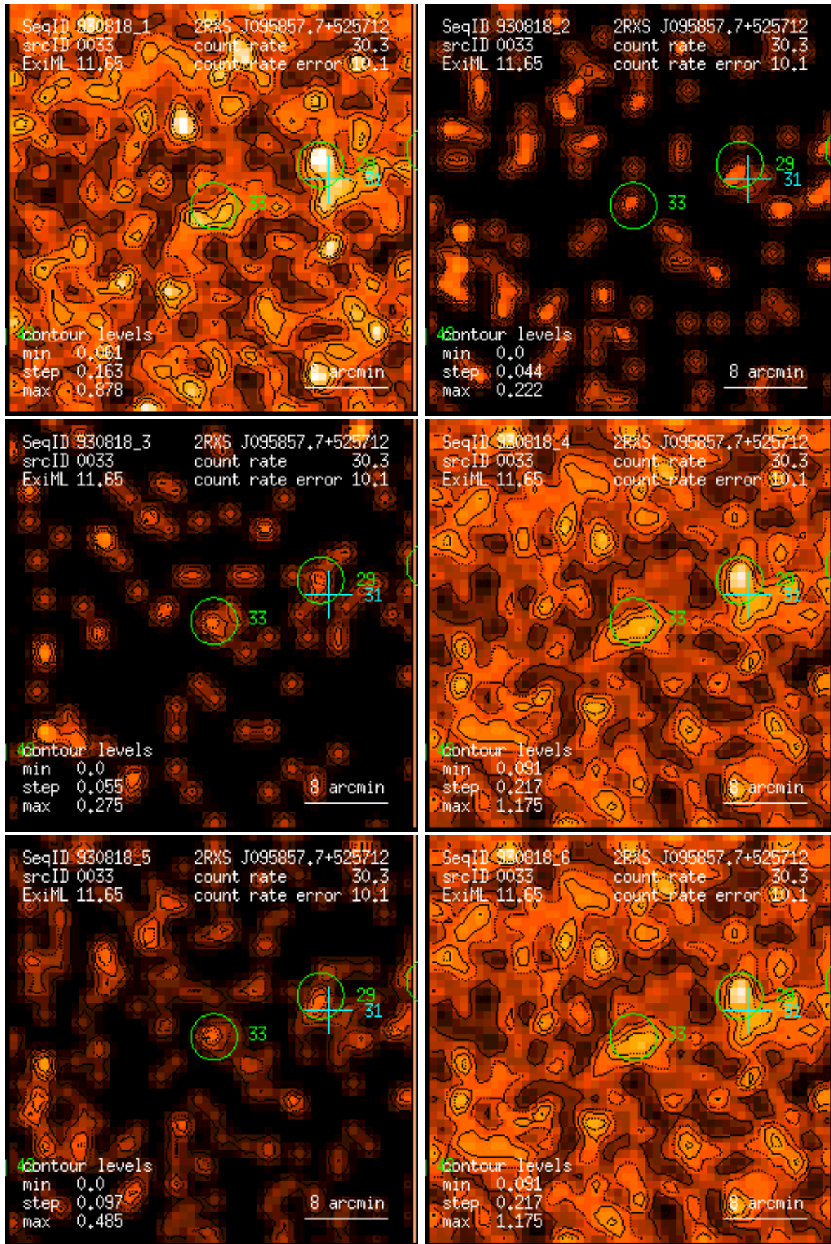
Figure 33: RASS 930818: detection 0033: band rate images, Gaussian filter: (1) PSPC channels 11 – 41, (2) 52 – 90, (3) 91 – 201, (4) 11 – 235, (5) 52 – 201, (6) 11 – 201. Broad band rates in counts/ks. Band rate contour levels in counts/ks/arcmin 2 .
