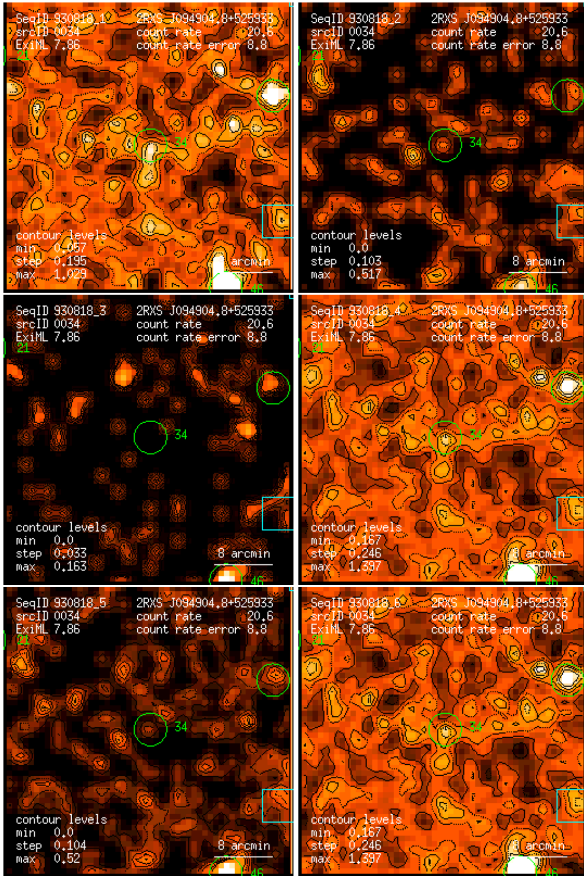
Figure 34: RASS 930818: detection 0034: band rate images, Gaussian filter: (1) PSPC channels 11 – 41, (2) 52 – 90, (3) 91 – 201, (4) 11 – 235, (5) 52 – 201, (6) 11 – 201. Broad band rates in counts/ks. Band rate contour levels in counts/ks/arcmin 2 .
