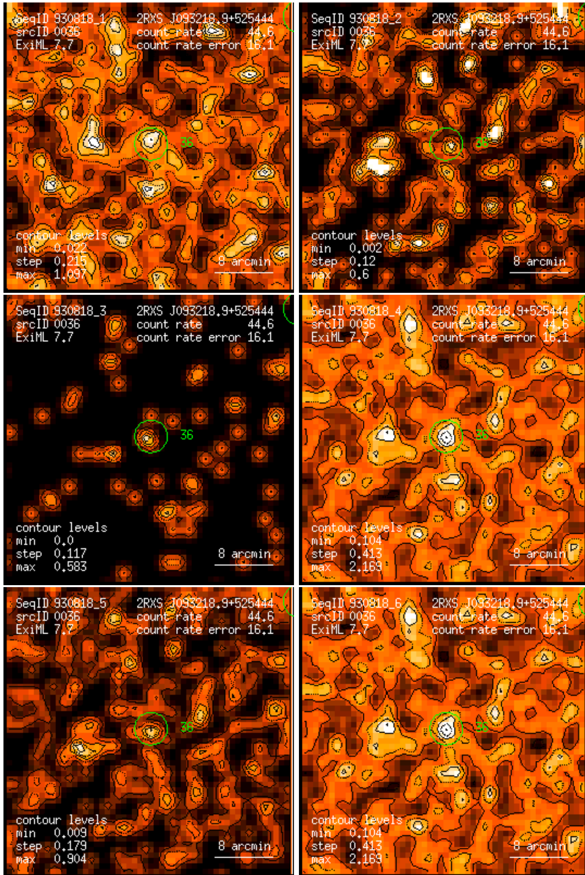
Figure 36: RASS 930818: detection 0036: band rate images, Gaussian filter: (1) PSPC channels 11 – 41, (2) 52 – 90, (3) 91 – 201, (4) 11 – 235, (5) 52 – 201, (6) 11 – 201. Broad band rates in counts/ks. Band rate contour levels in counts/ks/arcmin 2 .
