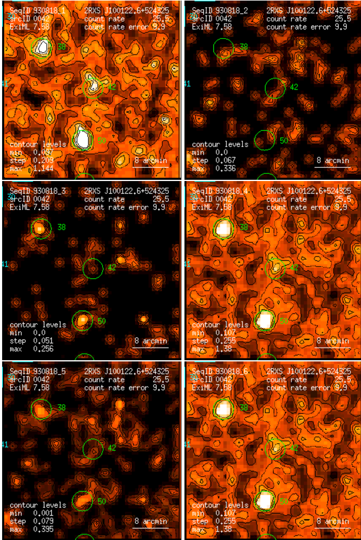
Figure 42: RASS 930818: detection 0042: band rate images, Gaussian filter: (1) PSPC channels 11 – 41, (2) 52 – 90, (3) 91 – 201, (4) 11 – 235, (5) 52 – 201, (6) 11 – 201. Broad band rates in counts/ks. Band rate contour levels in counts/ks/arcmin 2 .
