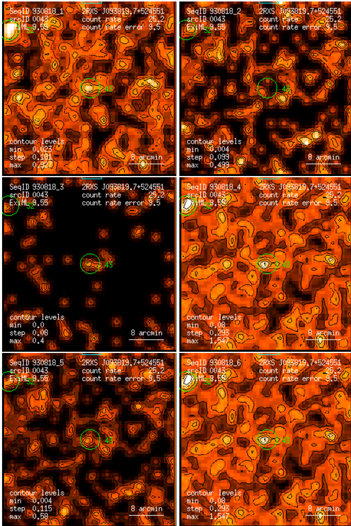
Figure 43: RASS 930818: detection 0043: band rate images, Gaussian filter: (1) PSPC channels 11 – 41, (2) 52 – 90, (3) 91 – 201, (4) 11 – 235, (5) 52 – 201, (6) 11 – 201. Broad band rates in counts/ks. Band rate contour levels in counts/ks/arcmin 2 .
