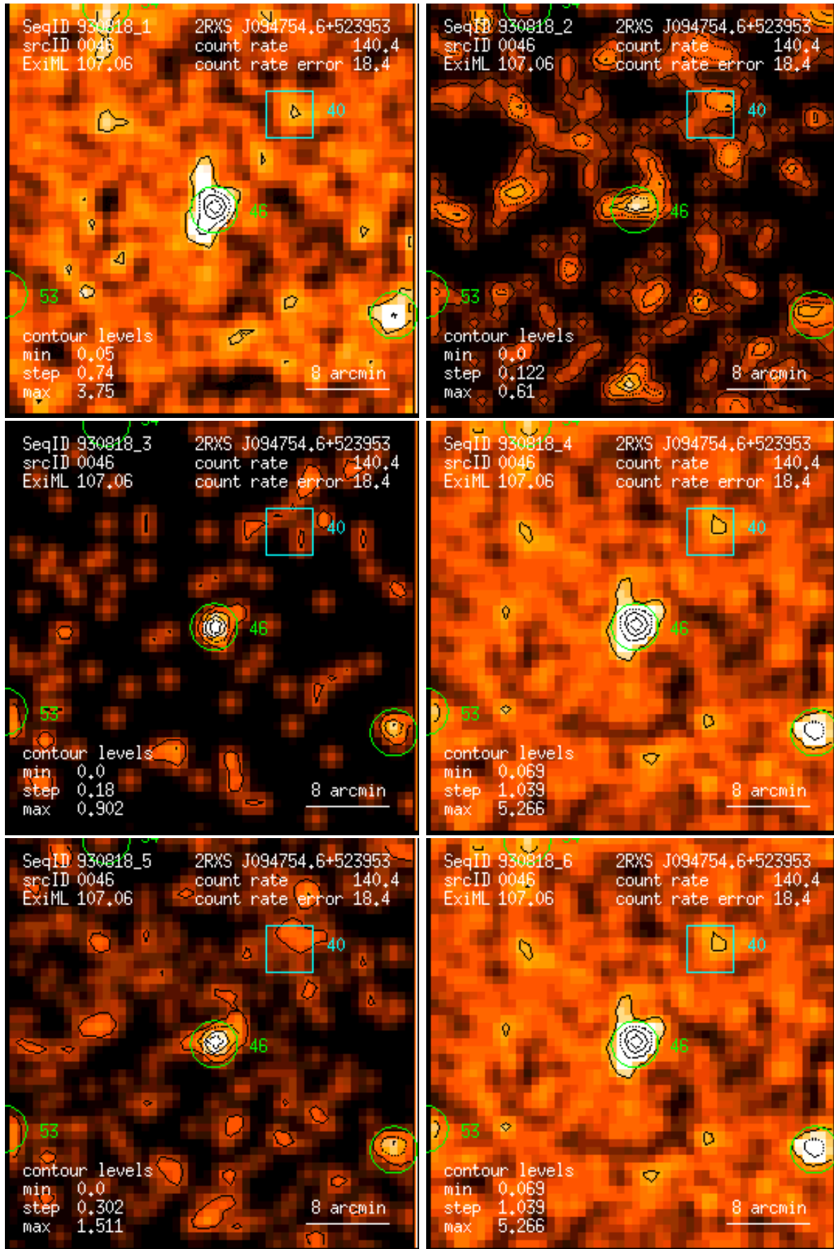
Figure 46: RASS 930818: detection 0046: band rate images, Gaussian filter: (1) PSPC channels 11 – 41, (2) 52 – 90, (3) 91 – 201, (4) 11 – 235, (5) 52 – 201, (6) 11 – 201. Broad band rates in counts/ks. Band rate contour levels in counts/ks/arcmin 2 .
