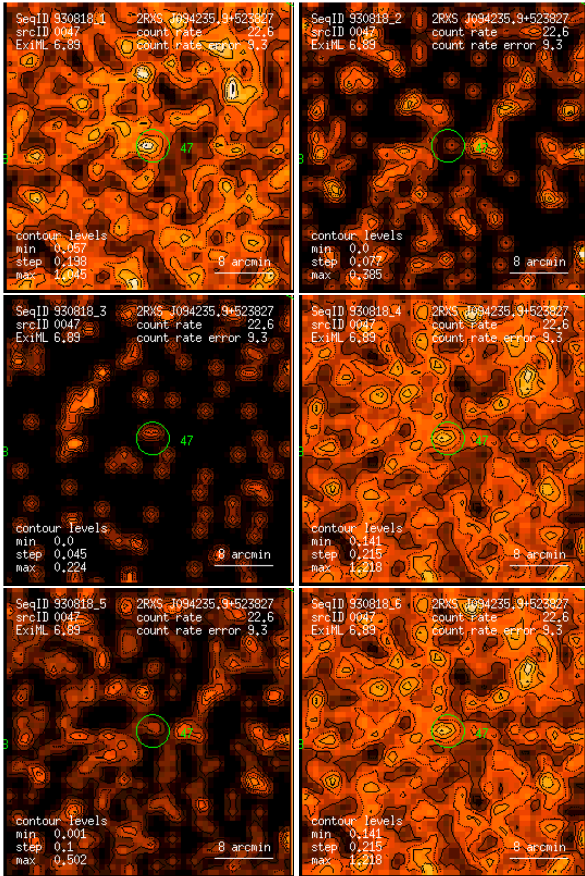
Figure 47: RASS 930818: detection 0047: band rate images, Gaussian filter: (1) PSPC channels 11 – 41, (2) 52 – 90, (3) 91 – 201, (4) 11 – 235, (5) 52 – 201, (6) 11 – 201. Broad band rates in counts/ks. Band rate contour levels in counts/ks/arcmin 2 .
