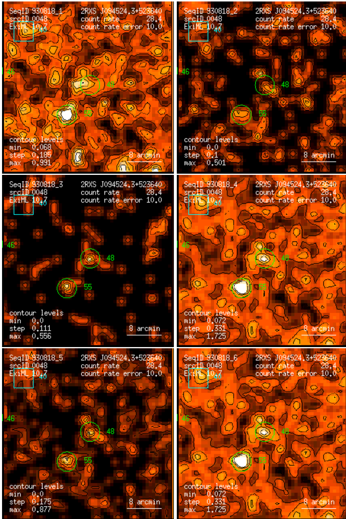
Figure 48: RASS 930818: detection 0048: band rate images, Gaussian filter: (1) PSPC channels 11 – 41, (2) 52 – 90, (3) 91 – 201, (4) 11 – 235, (5) 52 – 201, (6) 11 – 201. Broad band rates in counts/ks. Band rate contour levels in counts/ks/arcmin 2 .
