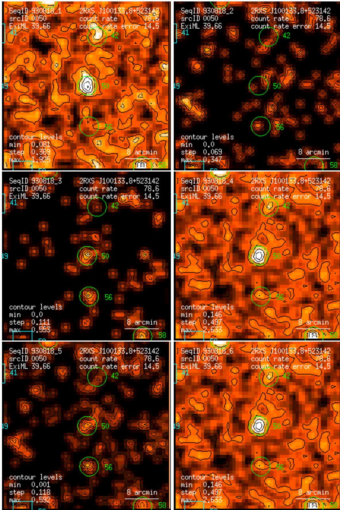
Figure 50: RASS 930818: detection 0050: band rate images, Gaussian filter: (1) PSPC channels 11 – 41, (2) 52 – 90, (3) 91 – 201, (4) 11 – 235, (5) 52 – 201, (6) 11 – 201. Broad band rates in counts/ks. Band rate contour levels in counts/ks/arcmin 2 .
