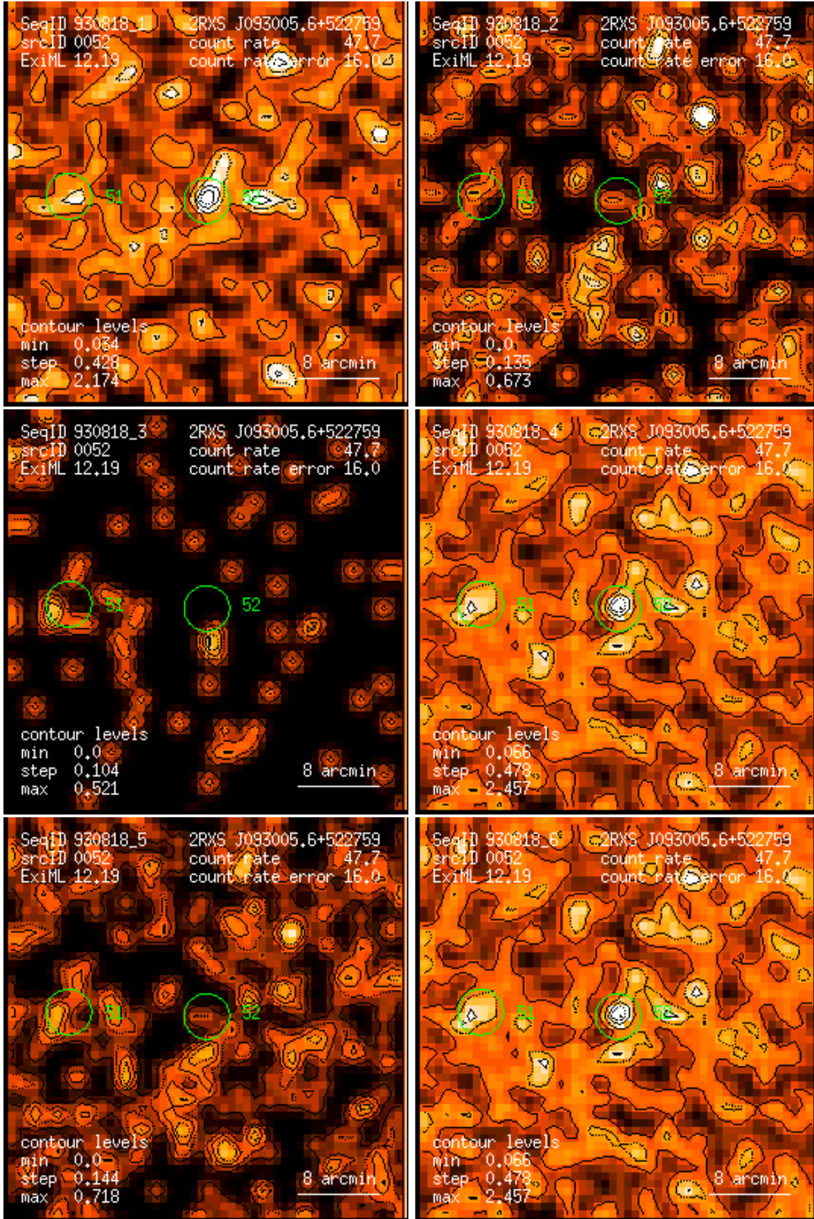
Figure 52: RASS 930818: detection 0052: band rate images, Gaussian filter: (1) PSPC channels 11 – 41, (2) 52 – 90, (3) 91 – 201, (4) 11 – 235, (5) 52 – 201, (6) 11 – 201. Broad band rates in counts/ks. Band rate contour levels in counts/ks/arcmin 2 .
