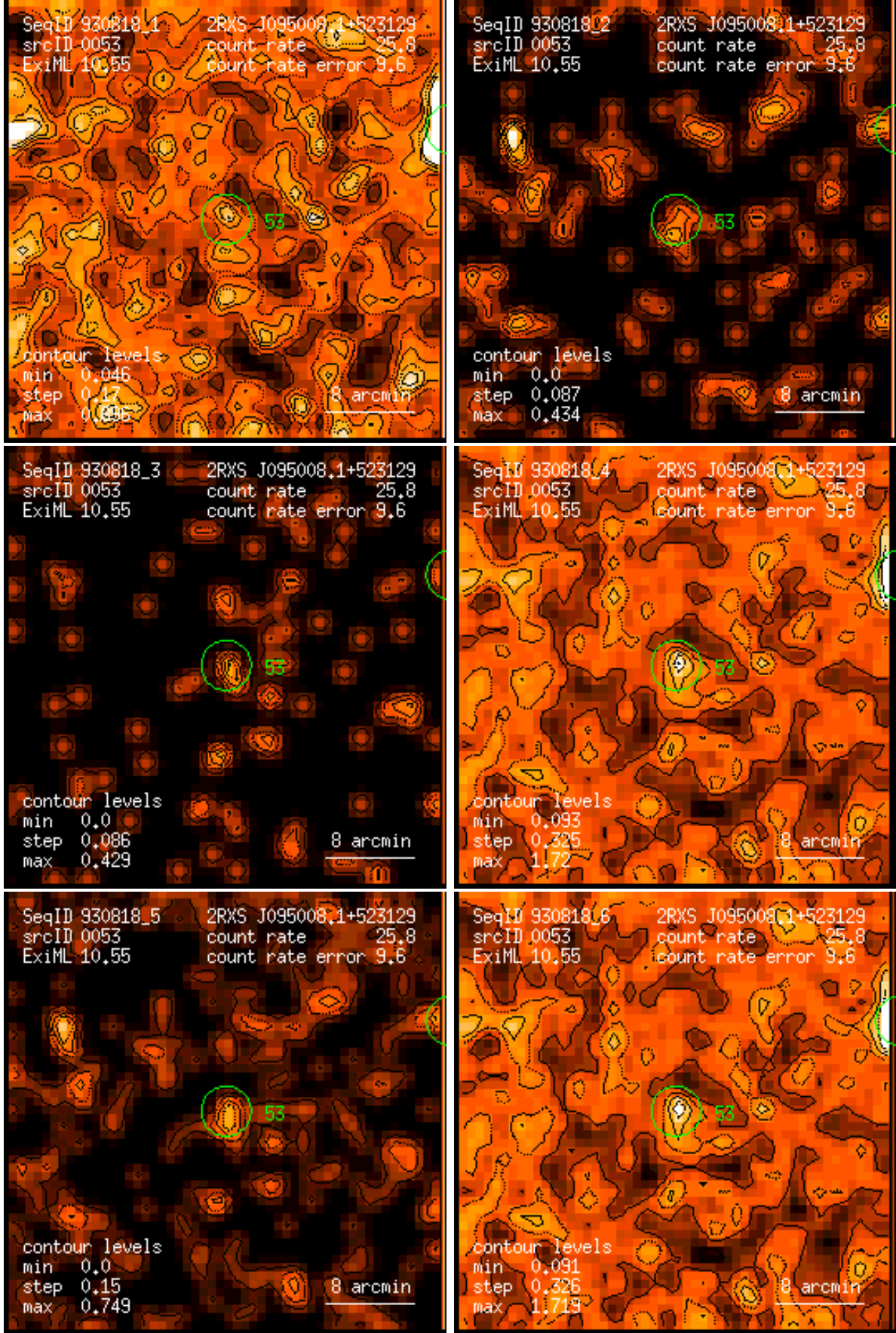
Figure 53: RASS 930818: detection 0053: band rate images, Gaussian filter: (1) PSPC channels 11 – 41, (2) 52 – 90, (3) 91 – 201, (4) 11 – 235, (5) 52 – 201, (6) 11 – 201. Broad band rates in counts/ks. Band rate contour levels in counts/ks/arcmin 2 .
