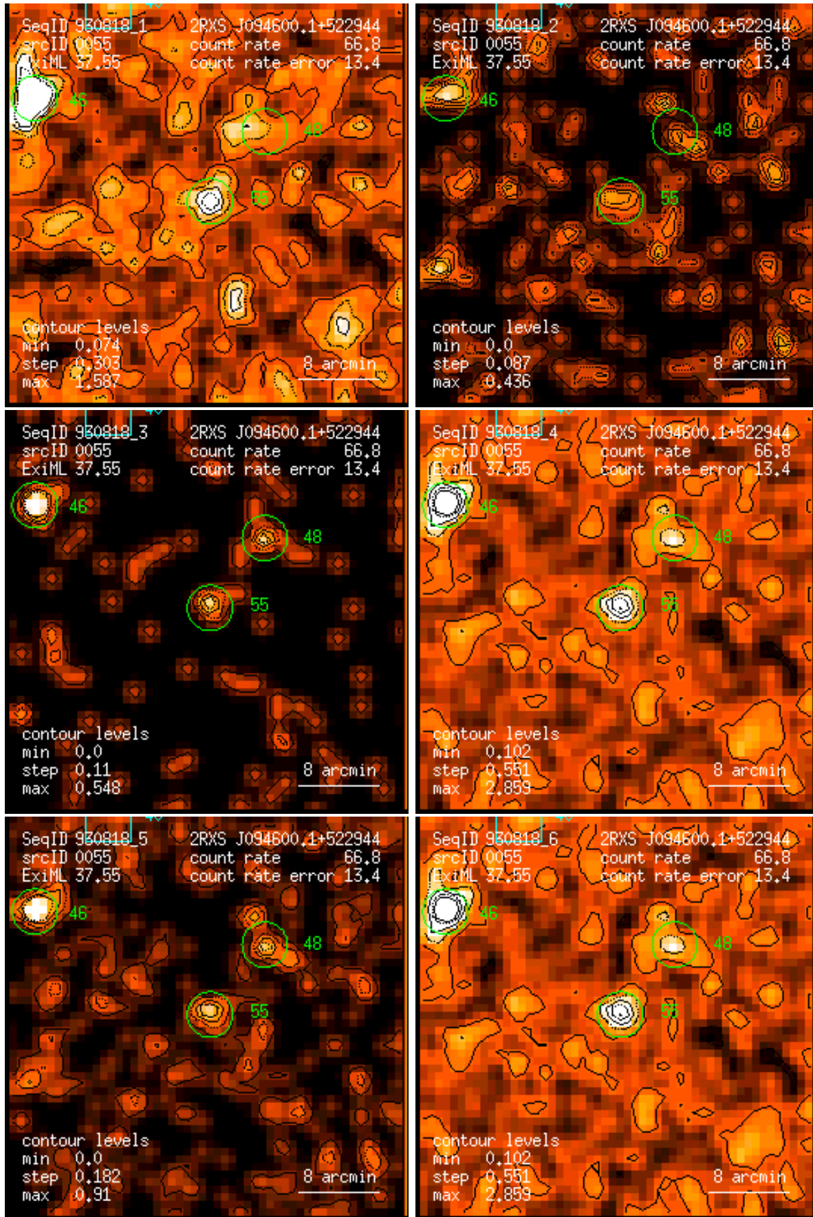
Figure 55: RASS 930818: detection 0055: band rate images, Gaussian filter: (1) PSPC channels 11 – 41, (2) 52 – 90, (3) 91 – 201, (4) 11 – 235, (5) 52 – 201, (6) 11 – 201. Broad band rates in counts/ks. Band rate contour levels in counts/ks/arcmin 2 .
