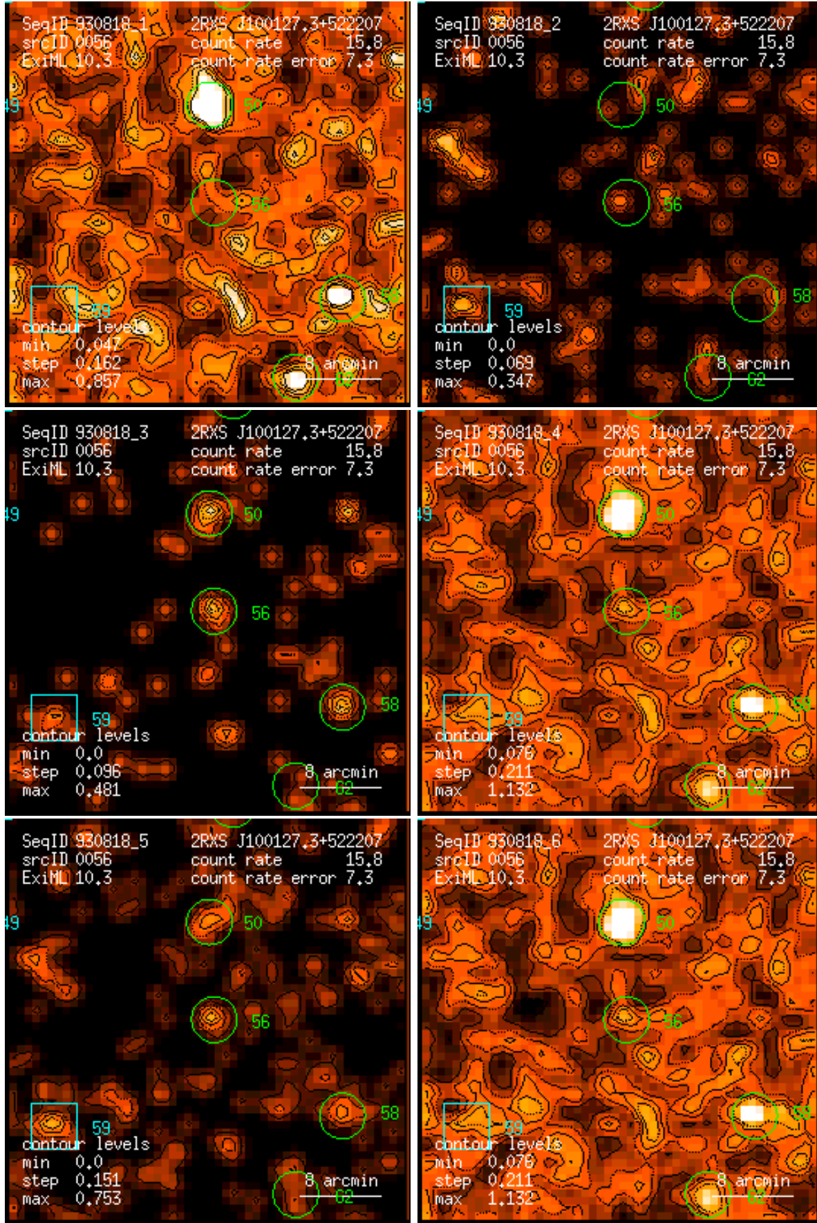
Figure 56: RASS 930818: detection 0056: band rate images, Gaussian filter: (1) PSPC channels 11 – 41, (2) 52 – 90, (3) 91 – 201, (4) 11 – 235, (5) 52 – 201, (6) 11 – 201. Broad band rates in counts/ks. Band rate contour levels in counts/ks/arcmin 2 .
