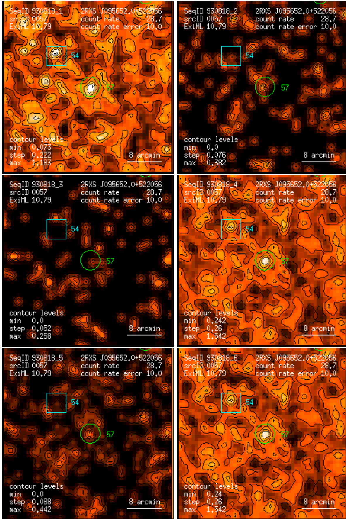
Figure 57: RASS 930818: detection 0057: band rate images, Gaussian filter: (1) PSPC channels 11 – 41, (2) 52 – 90, (3) 91 – 201, (4) 11 – 235, (5) 52 – 201, (6) 11 – 201. Broad band rates in counts/ks. Band rate contour levels in counts/ks/arcmin 2 .
