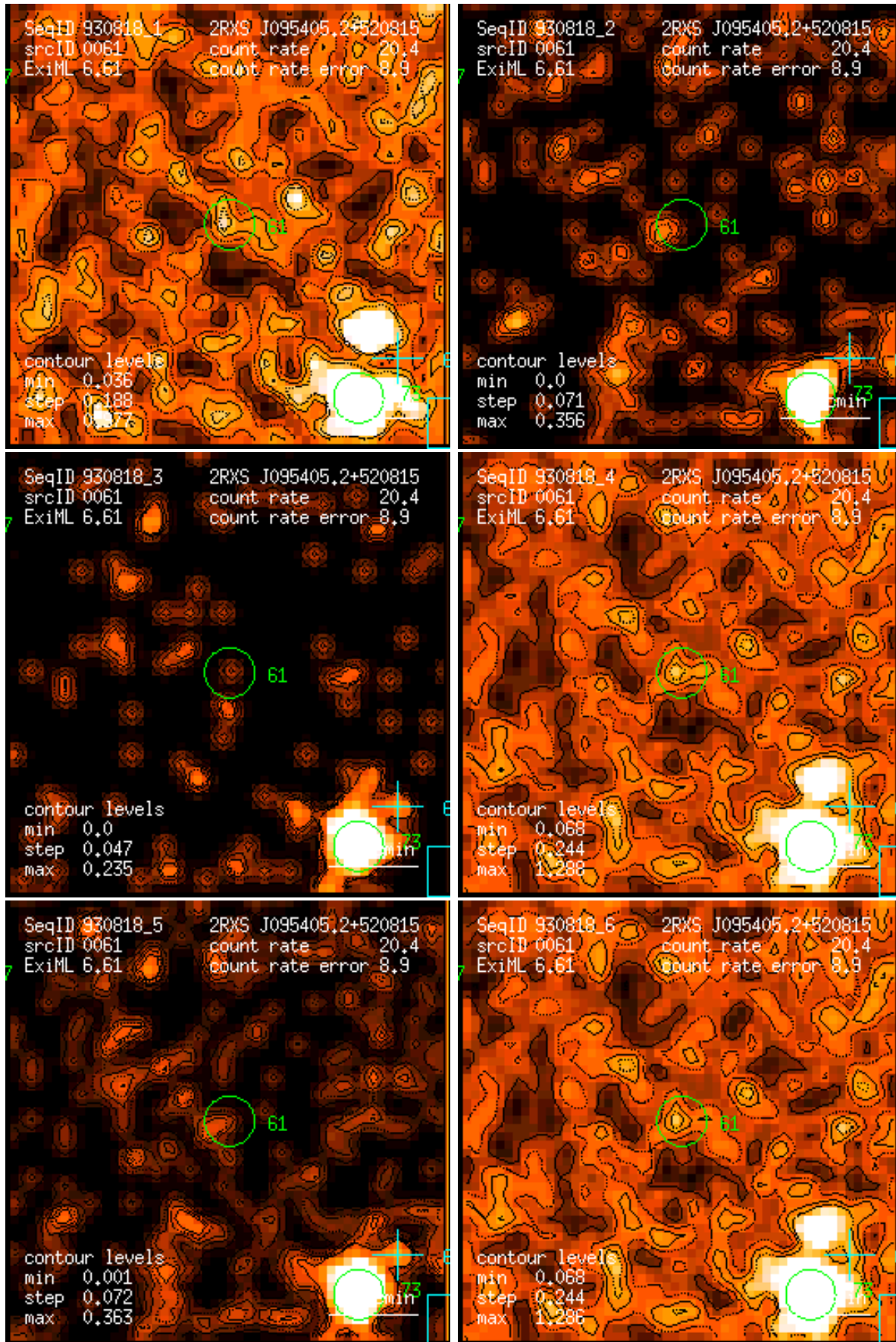
Figure 61: RASS 930818: detection 0061: band rate images, Gaussian filter: (1) PSPC channels 11 – 41, (2) 52 – 90, (3) 91 – 201, (4) 11 – 235, (5) 52 – 201, (6) 11 – 201. Broad band rates in counts/ks. Band rate contour levels in counts/ks/arcmin 2 .
