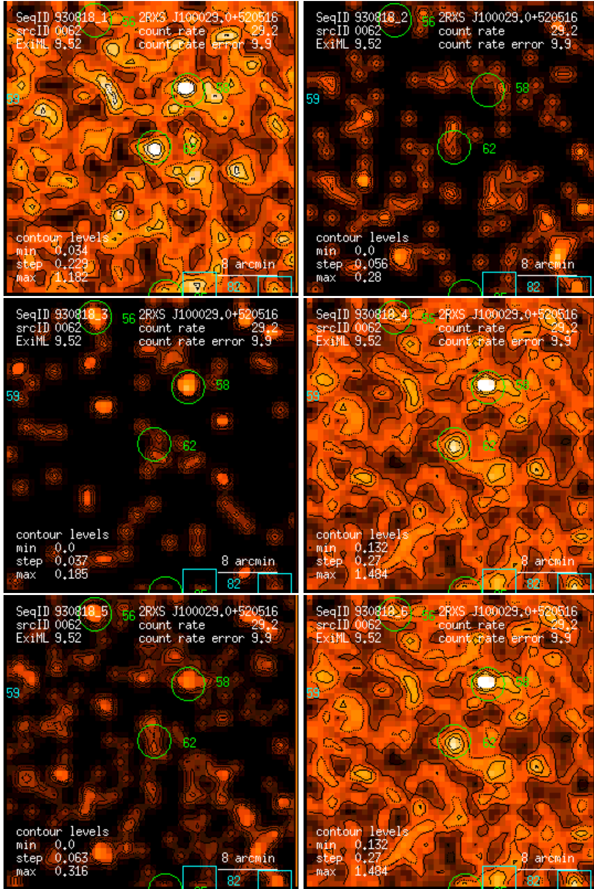
Figure 62: RASS 930818: detection 0062: band rate images, Gaussian filter: (1) PSPC channels 11 – 41, (2) 52 – 90, (3) 91 – 201, (4) 11 – 235, (5) 52 – 201, (6) 11 – 201. Broad band rates in counts/ks. Band rate contour levels in counts/ks/arcmin 2 .
