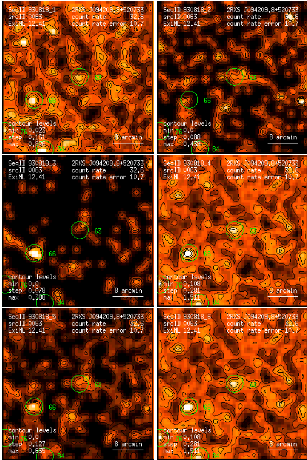
Figure 63: RASS 930818: detection 0063: band rate images, Gaussian filter: (1) PSPC channels 11 – 41, (2) 52 – 90, (3) 91 – 201, (4) 11 – 235, (5) 52 – 201, (6) 11 – 201. Broad band rates in counts/ks. Band rate contour levels in counts/ks/arcmin 2 .
