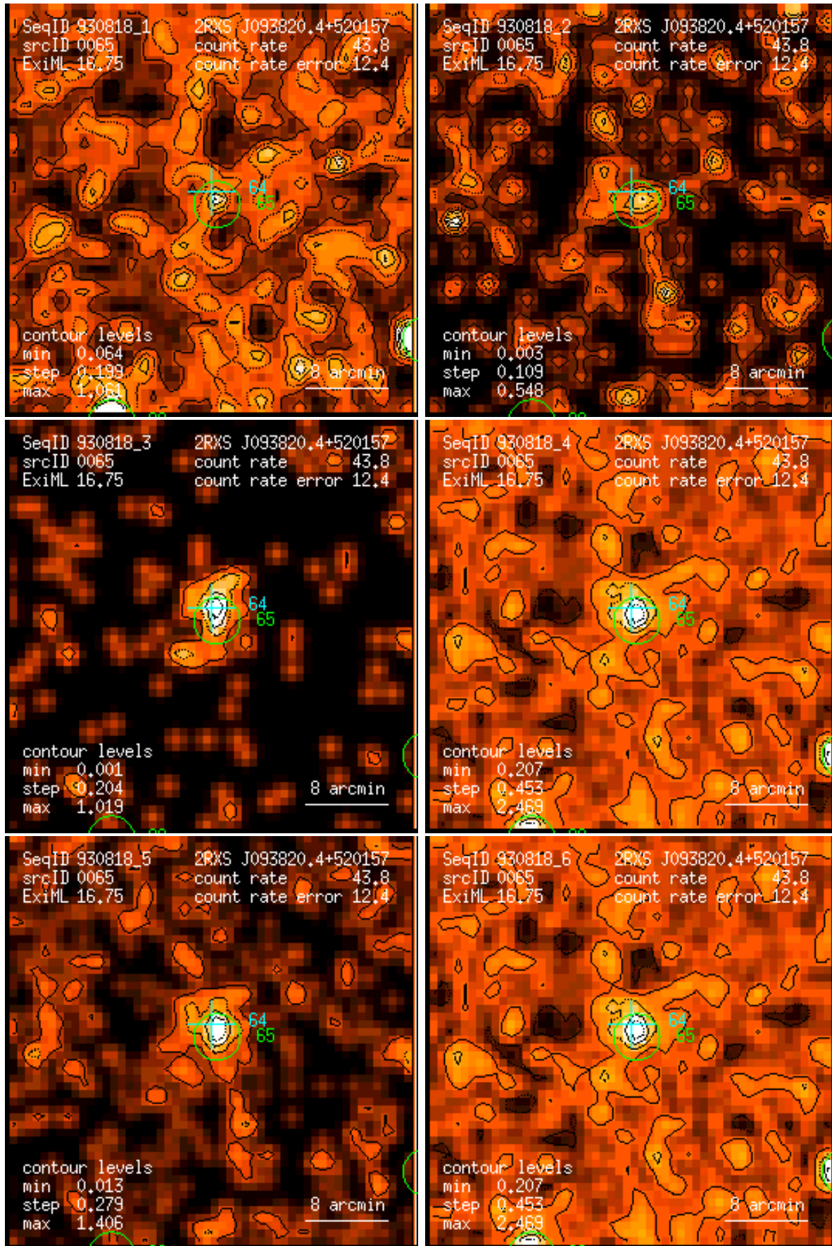
Figure 65: RASS 930818: detection 0065: band rate images, Gaussian filter: (1) PSPC channels 11 – 41, (2) 52 – 90, (3) 91 – 201, (4) 11 – 235, (5) 52 – 201, (6) 11 – 201. Broad band rates in counts/ks. Band rate contour levels in counts/ks/arcmin 2 .
