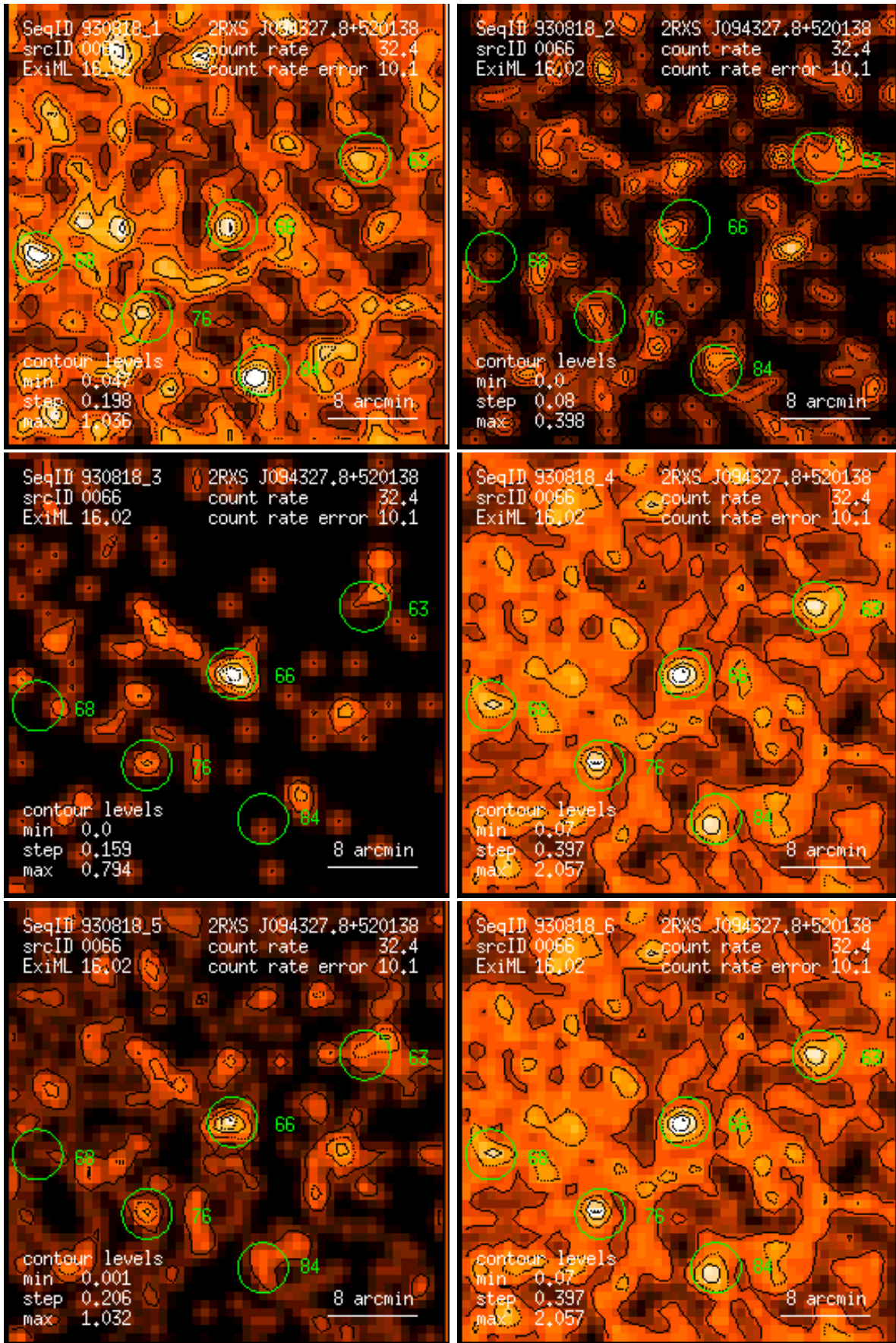
Figure 66: RASS 930818: detection 0066: band rate images, Gaussian filter: (1) PSPC channels 11 – 41, (2) 52 – 90, (3) 91 – 201, (4) 11 – 235, (5) 52 – 201, (6) 11 – 201. Broad band rates in counts/ks. Band rate contour levels in counts/ks/arcmin 2 .
