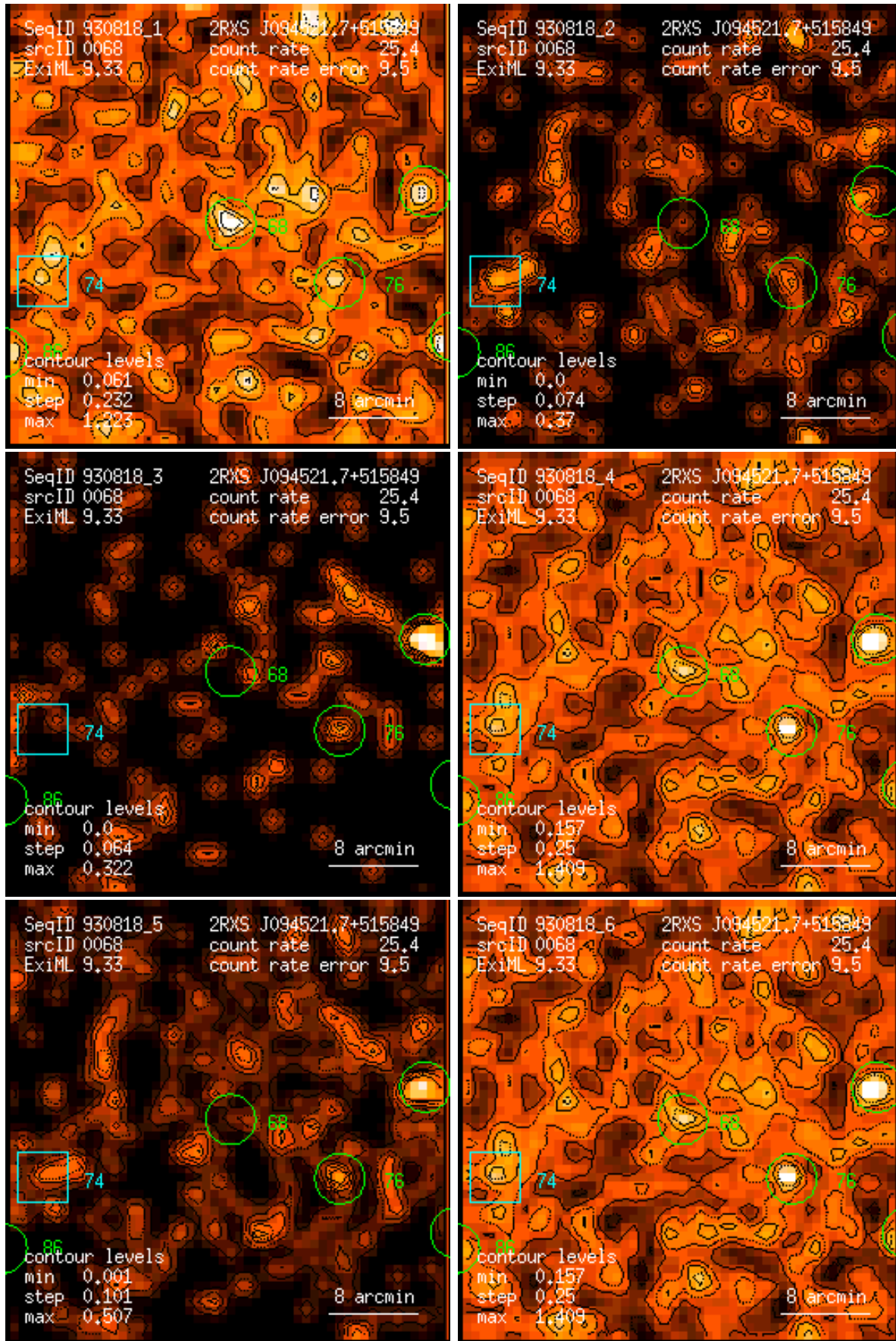
Figure 68: RASS 930818: detection 0068: band rate images, Gaussian filter: (1) PSPC channels 11 – 41, (2) 52 – 90, (3) 91 – 201, (4) 11 – 235, (5) 52 – 201, (6) 11 – 201. Broad band rates in counts/ks. Band rate contour levels in counts/ks/arcmin 2 .
