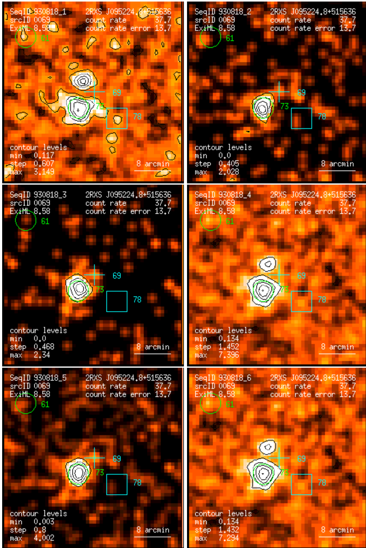
Figure 69: RASS 930818: detection 0069: band rate images, Gaussian filter: (1) PSPC channels 11 – 41, (2) 52 – 90, (3) 91 – 201, (4) 11 – 235, (5) 52 – 201, (6) 11 – 201. Broad band rates in counts/ks. Band rate contour levels in counts/ks/arcmin 2 .
