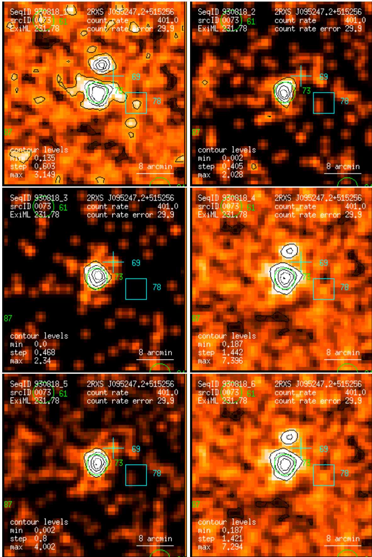
Figure 73: RASS 930818: detection 0073: band rate images, Gaussian filter: (1) PSPC channels 11 – 41, (2) 52 – 90, (3) 91 – 201, (4) 11 – 235, (5) 52 – 201, (6) 11 – 201. Broad band rates in counts/ks. Band rate contour levels in counts/ks/arcmin 2 .
