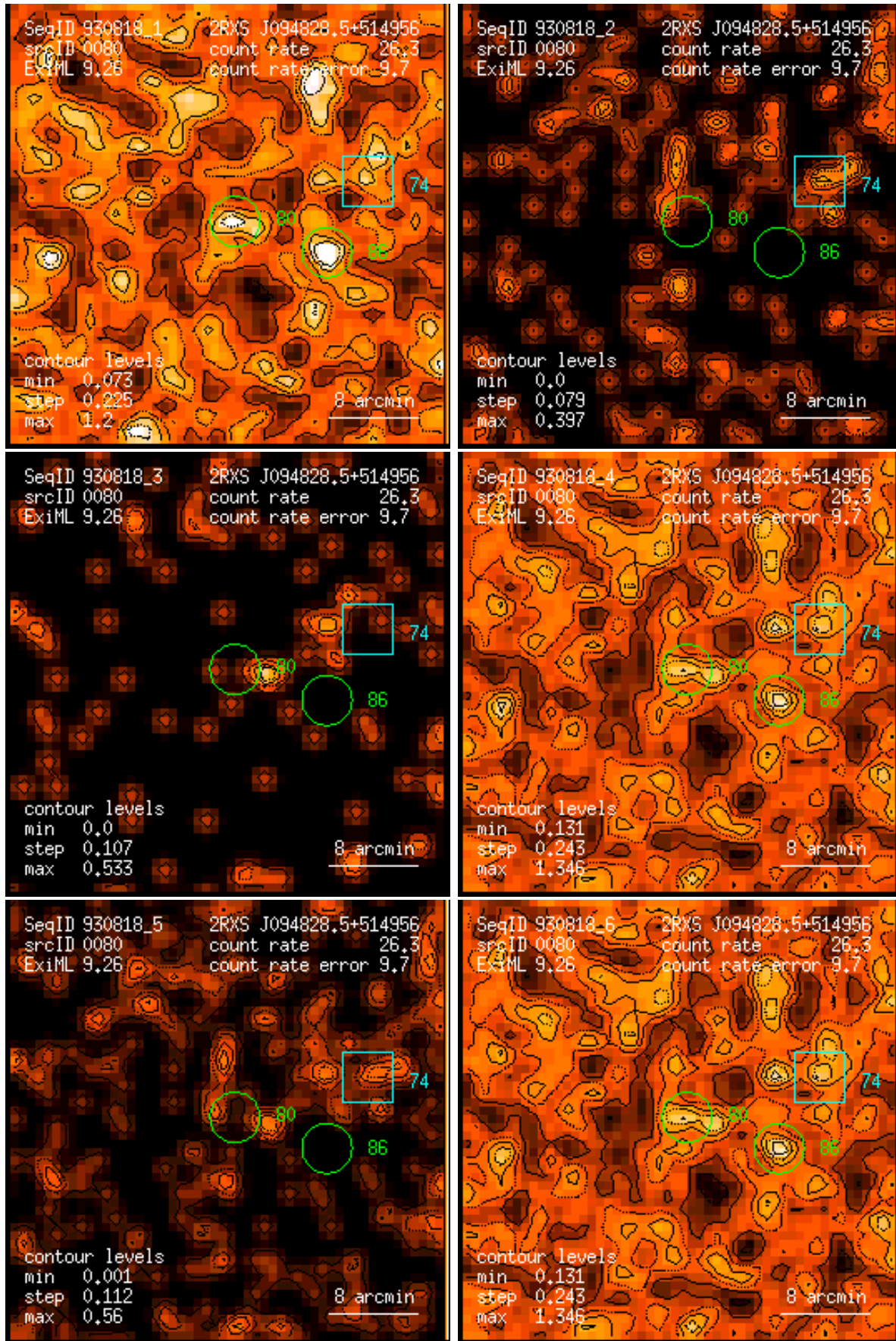
Figure 80: RASS 930818: detection 0080: band rate images, Gaussian filter: (1) PSPC channels 11 – 41, (2) 52 – 90, (3) 91 – 201, (4) 11 – 235, (5) 52 – 201, (6) 11 – 201. Broad band rates in counts/ks. Band rate contour levels in counts/ks/arcmin 2 .
