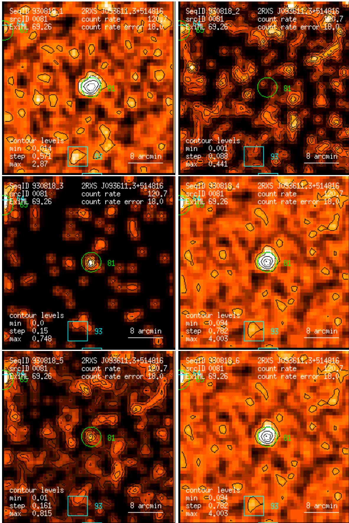
Figure 81: RASS 930818: detection 0081: band rate images, Gaussian filter: (1) PSPC channels 11 – 41, (2) 52 – 90, (3) 91 – 201, (4) 11 – 235, (5) 52 – 201, (6) 11 – 201. Broad band rates in counts/ks. Band rate contour levels in counts/ks/arcmin 2 .
