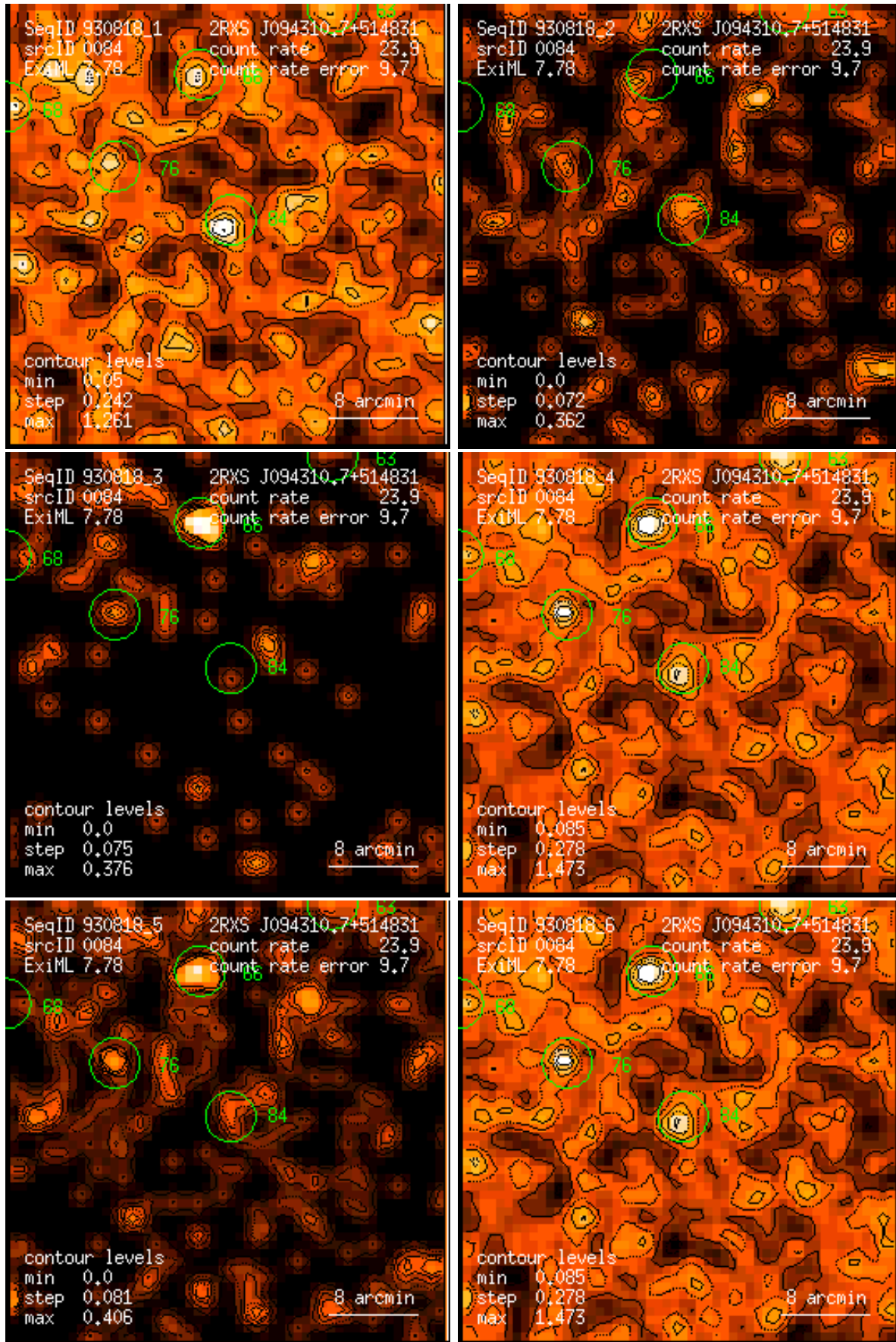
Figure 84: RASS 930818: detection 0084: band rate images, Gaussian filter: (1) PSPC channels 11 – 41, (2) 52 – 90, (3) 91 – 201, (4) 11 – 235, (5) 52 – 201, (6) 11 – 201. Broad band rates in counts/ks. Band rate contour levels in counts/ks/arcmin 2 .
