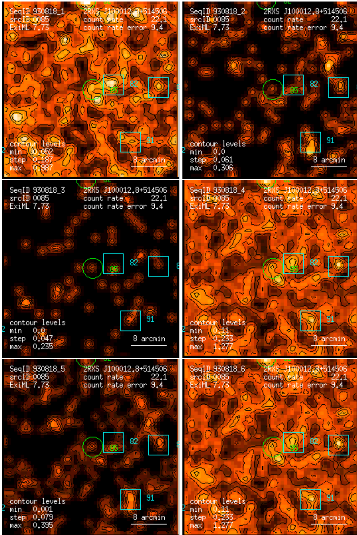
Figure 85: RASS 930818: detection 0085: band rate images, Gaussian filter: (1) PSPC channels 11 – 41, (2) 52 – 90, (3) 91 – 201, (4) 11 – 235, (5) 52 – 201, (6) 11 – 201. Broad band rates in counts/ks. Band rate contour levels in counts/ks/arcmin 2 .
